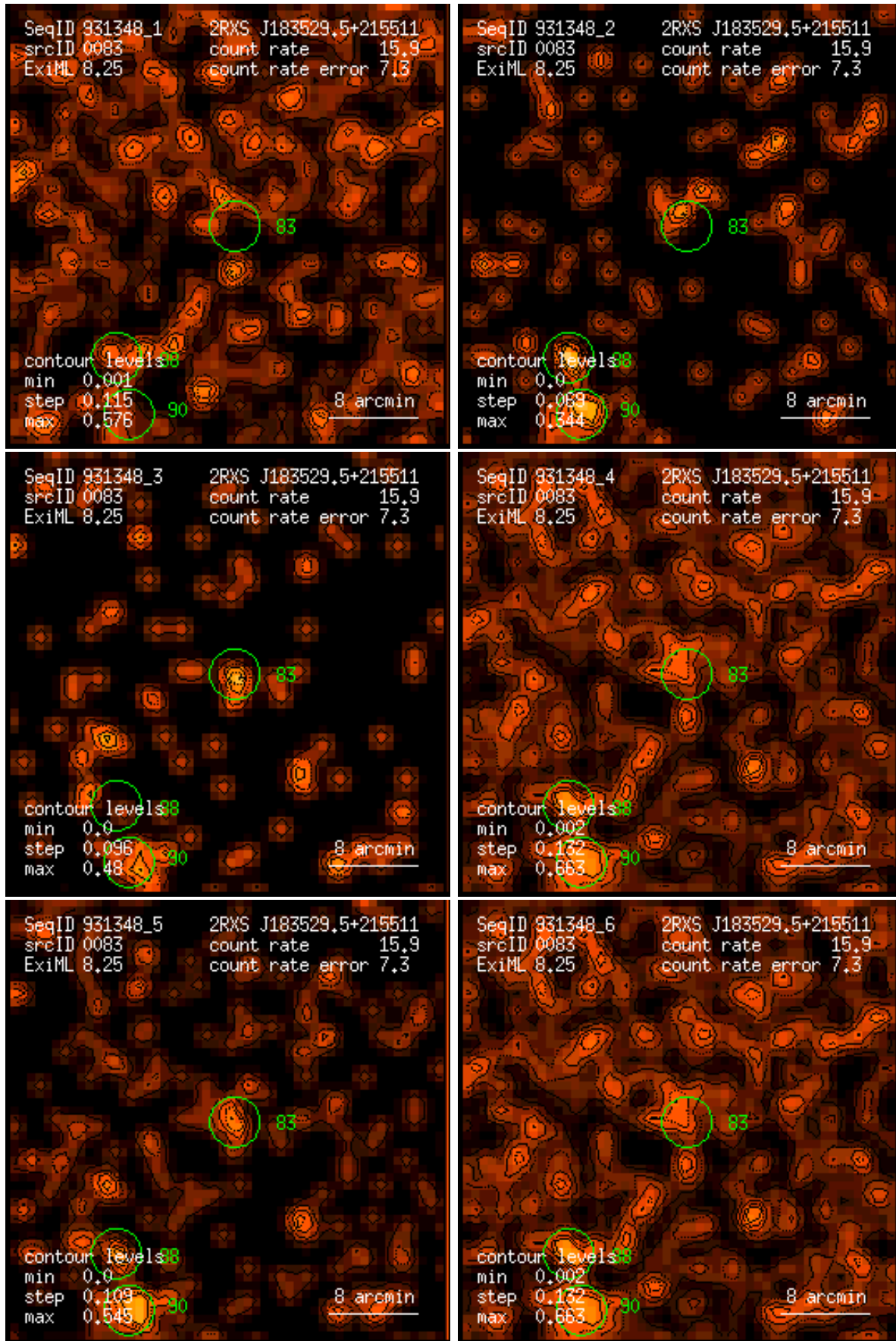
Figure 83: RASS 931348: detection 0083: band rate images, Gaussian filter: (1) PSPC channels 11 – 41, (2) 52 – 90, (3) 91 – 201, (4) 11 – 235, (5) 52 – 201, (6) 11 – 201. Broad band rates in counts/ks. Band rate contour levels in counts/ks/arcmin 2 .
