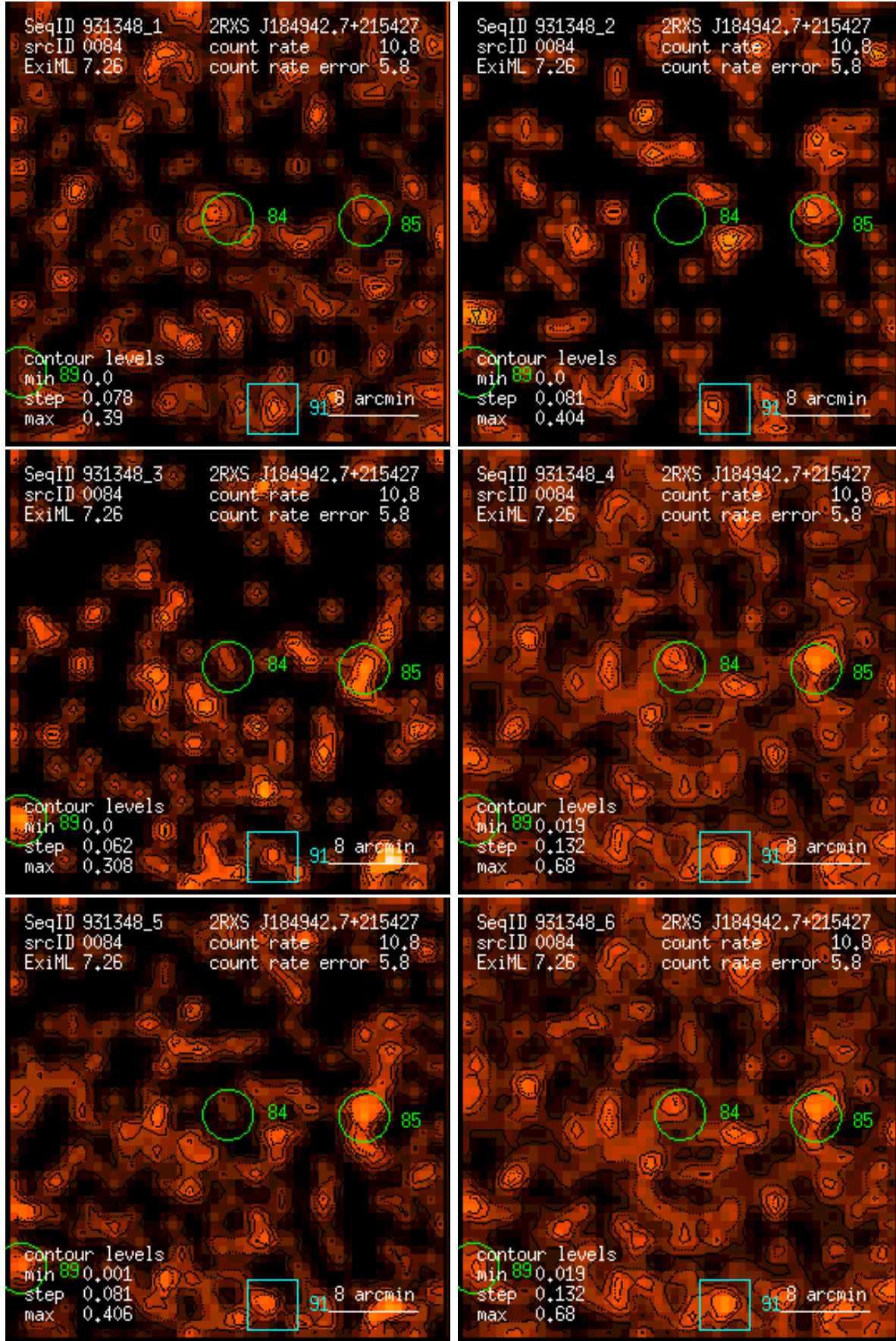
Figure 84: RASS 931348: detection 0084: band rate images, Gaussian filter: (1) PSPC channels 11 – 41, (2) 52 – 90, (3) 91 – 201, (4) 11 – 235, (5) 52 – 201, (6) 11 – 201. Broad band rates in counts/ks. Band rate contour levels in counts/ks/arcmin 2 .
