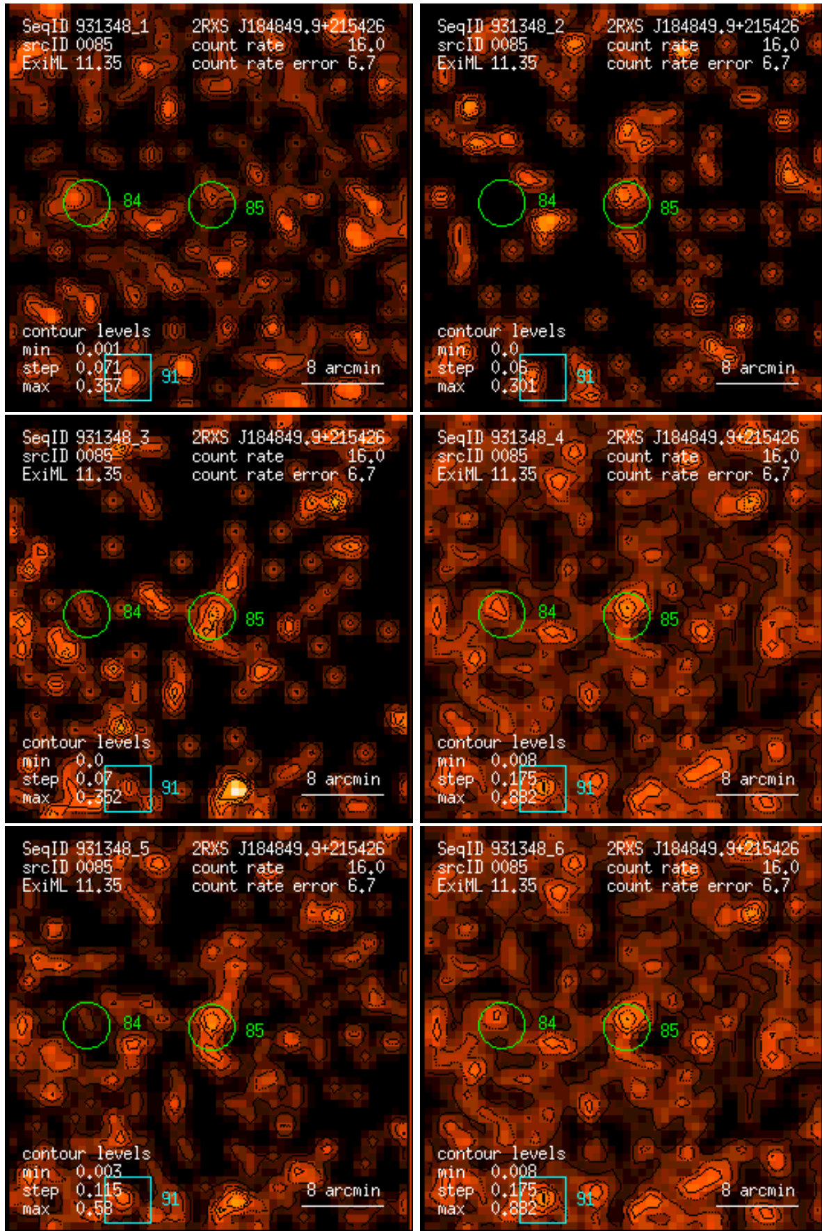
Figure 85: RASS 931348: detection 0085: band rate images, Gaussian filter: (1) PSPC channels 11 – 41, (2) 52 – 90, (3) 91 – 201, (4) 11 – 235, (5) 52 – 201, (6) 11 – 201. Broad band rates in counts/ks. Band rate contour levels in counts/ks/arcmin 2 .
