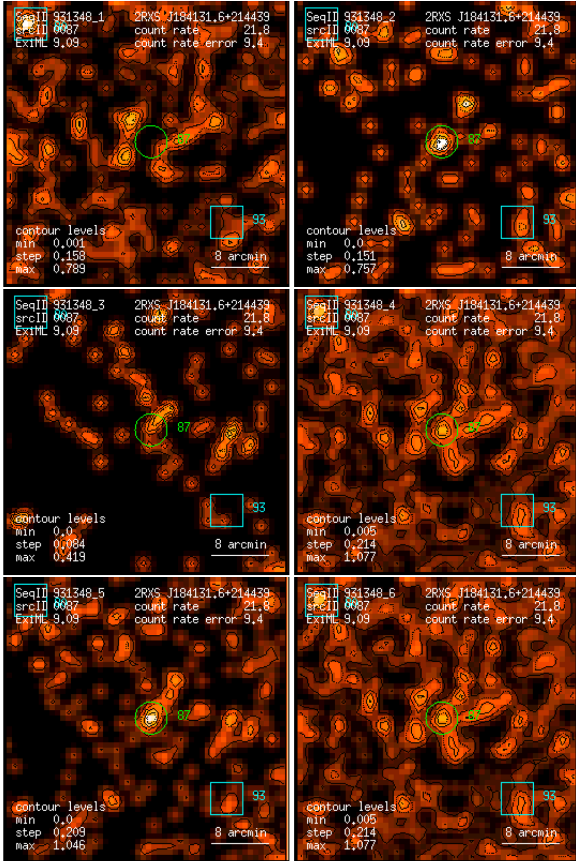
Figure 87: RASS 931348: detection 0087: band rate images, Gaussian filter: (1) PSPC channels 11 – 41, (2) 52 – 90, (3) 91 – 201, (4) 11 – 235, (5) 52 – 201, (6) 11 – 201. Broad band rates in counts/ks. Band rate contour levels in counts/ks/arcmin 2 .
