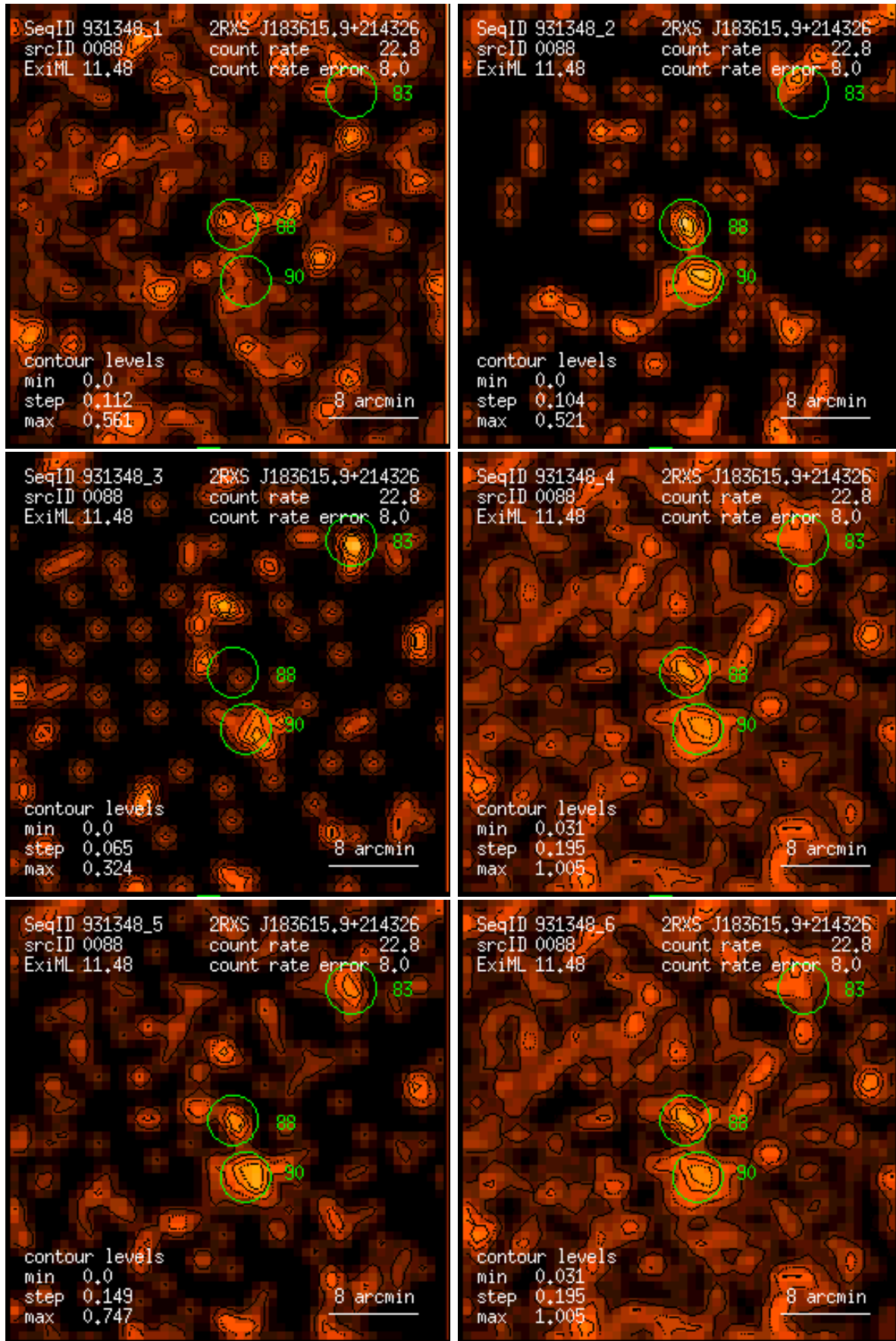
Figure 88: RASS 931348: detection 0088: band rate images, Gaussian filter: (1) PSPC channels 11 – 41, (2) 52 – 90, (3) 91 – 201, (4) 11 – 235, (5) 52 – 201, (6) 11 – 201. Broad band rates in counts/ks. Band rate contour levels in counts/ks/arcmin 2 .
