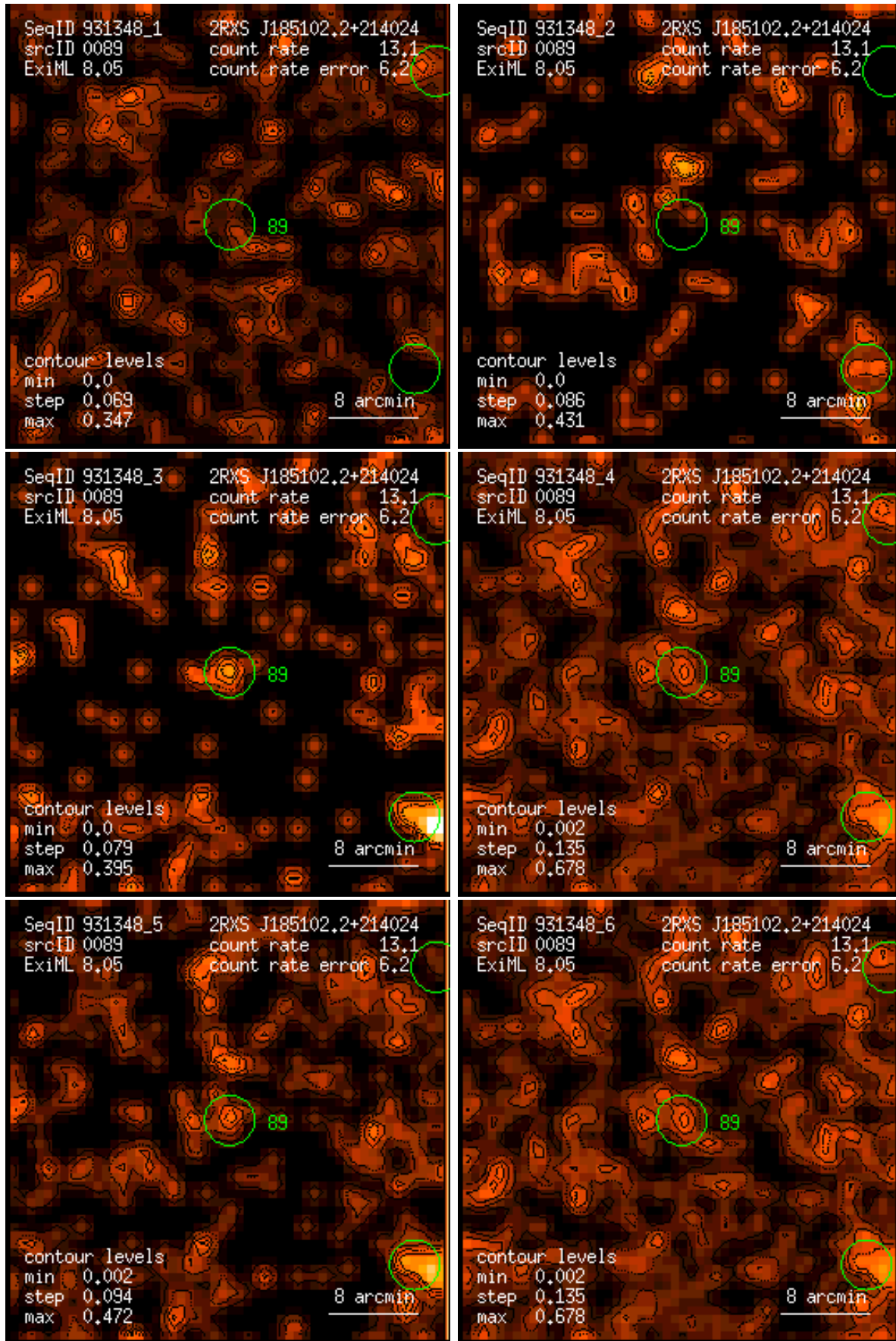
Figure 89: RASS 931348: detection 0089: band rate images, Gaussian filter: (1) PSPC channels 11 – 41, (2) 52 – 90, (3) 91 – 201, (4) 11 – 235, (5) 52 – 201, (6) 11 – 201. Broad band rates in counts/ks. Band rate contour levels in counts/ks/arcmin 2 .
