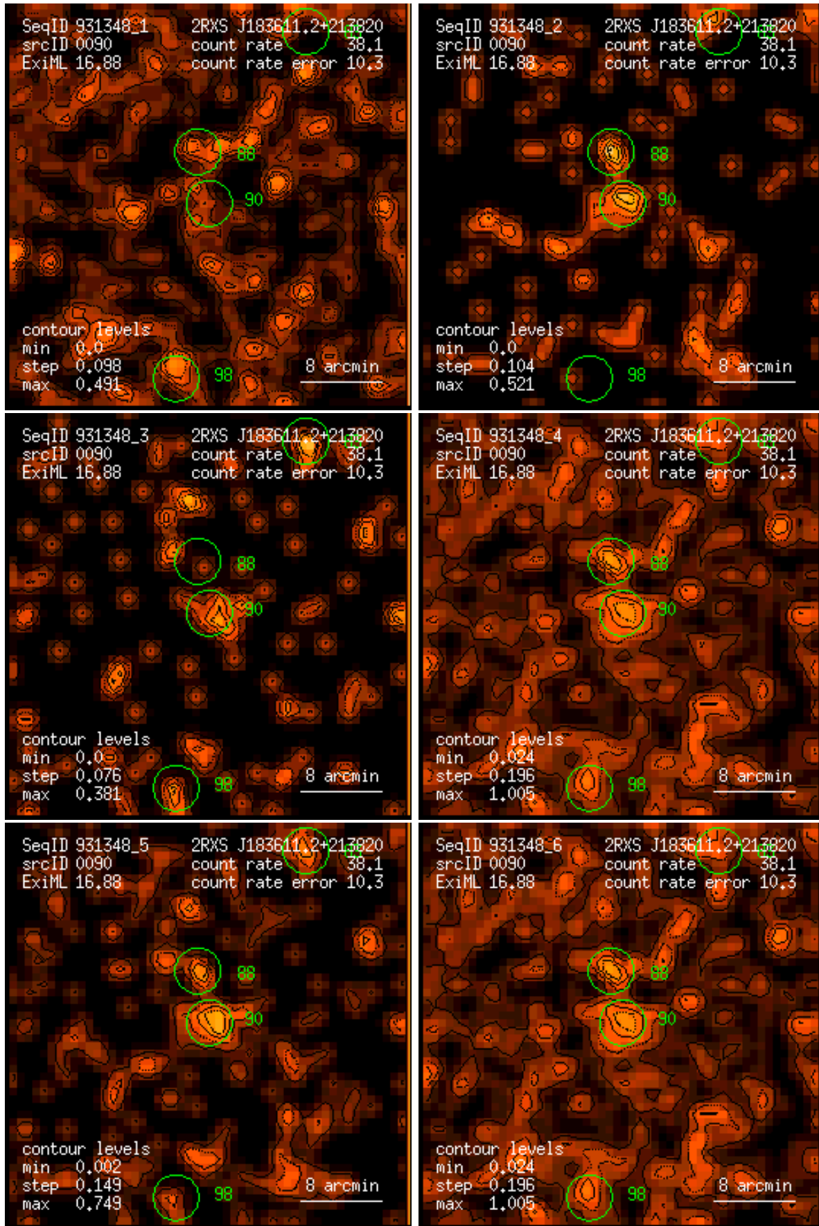
Figure 90: RASS 931348: detection 0090: band rate images, Gaussian filter: (1) PSPC channels 11 – 41, (2) 52 – 90, (3) 91 – 201, (4) 11 – 235, (5) 52 – 201, (6) 11 – 201. Broad band rates in counts/ks. Band rate contour levels in counts/ks/arcmin 2 .
