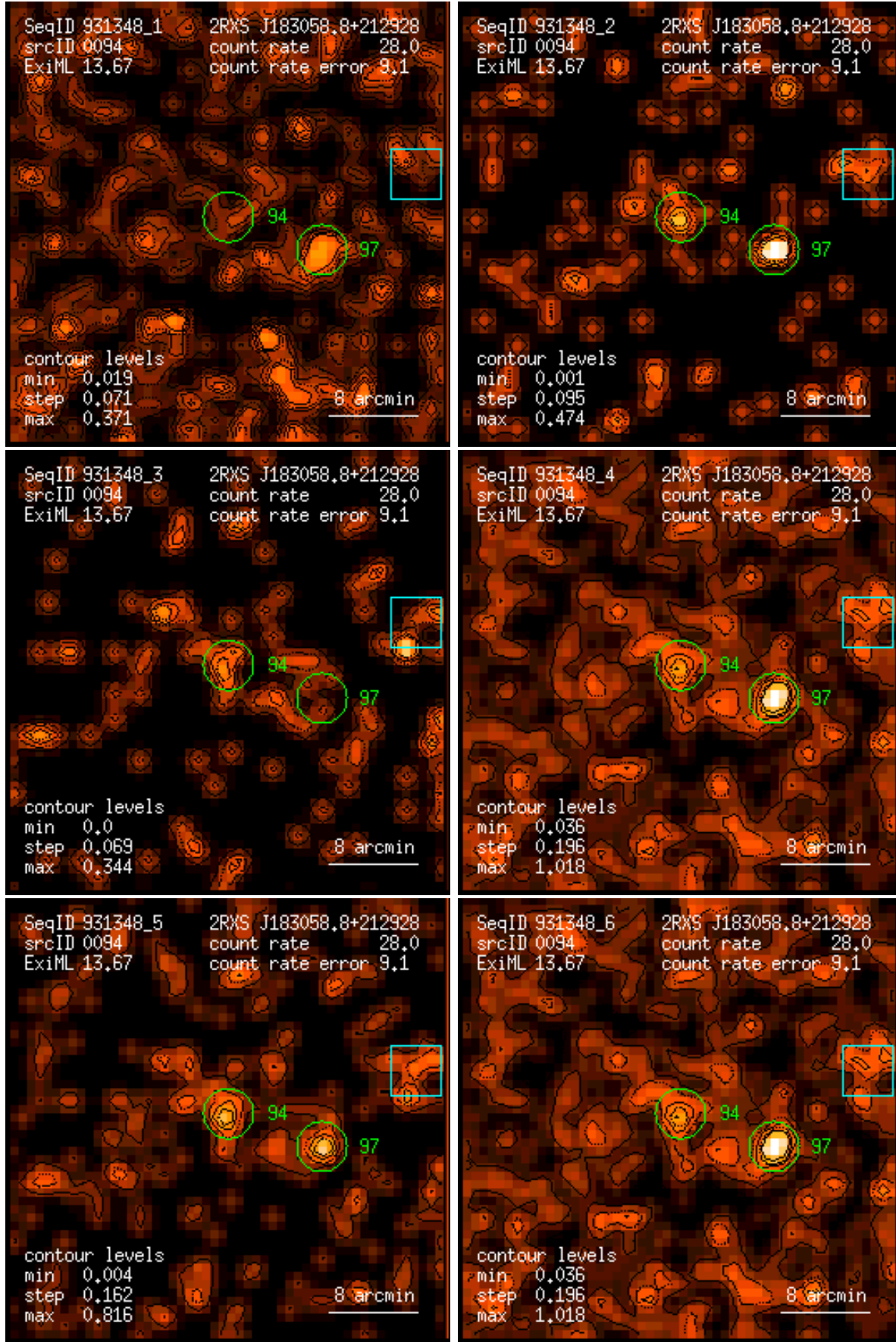
Figure 94: RASS 931348: detection 0094: band rate images, Gaussian filter: (1) PSPC channels 11 – 41, (2) 52 – 90, (3) 91 – 201, (4) 11 – 235, (5) 52 – 201, (6) 11 – 201. Broad band rates in counts/ks. Band rate contour levels in counts/ks/arcmin 2 .
