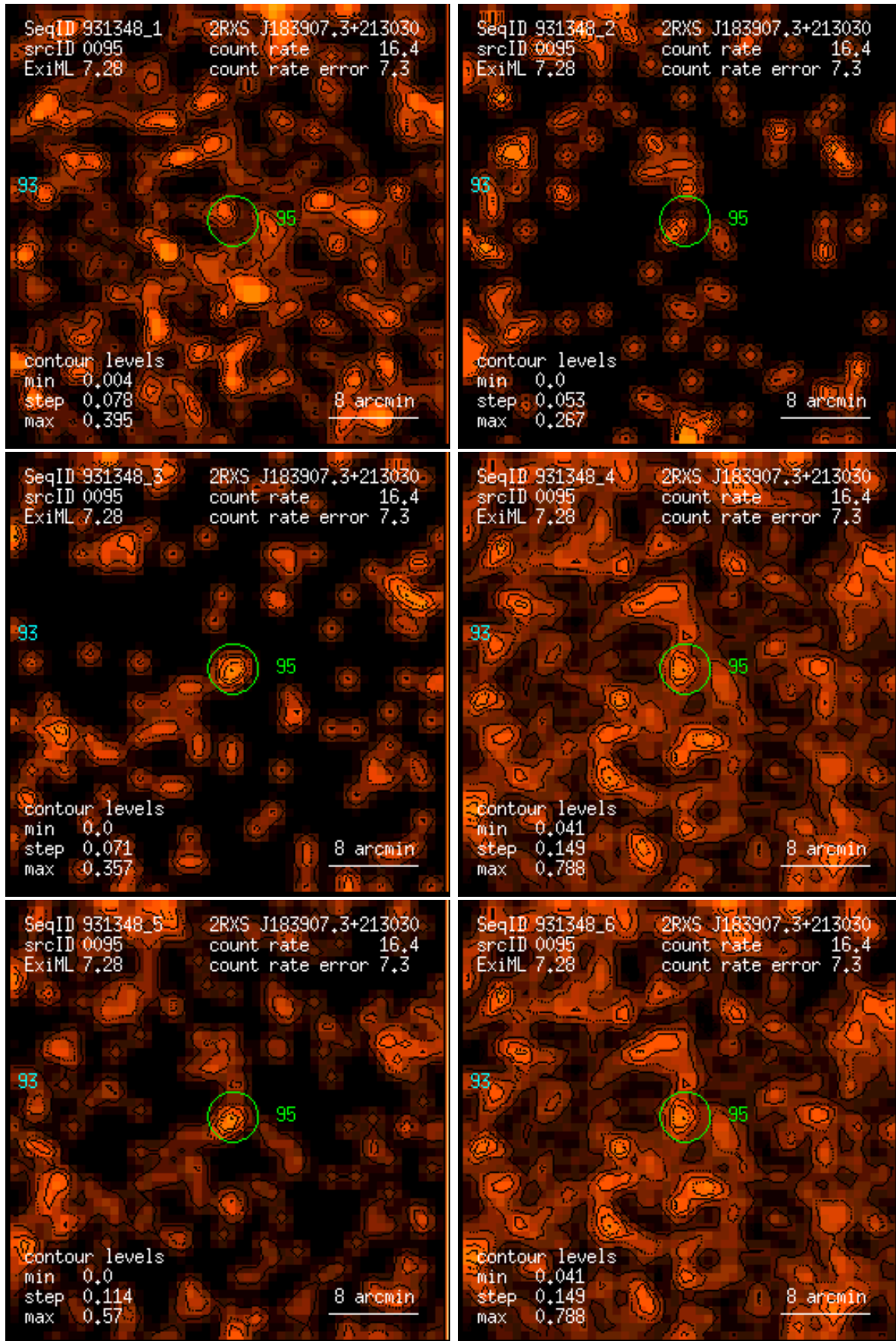
Figure 95: RASS 931348: detection 0095: band rate images, Gaussian filter: (1) PSPC channels 11 – 41, (2) 52 – 90, (3) 91 – 201, (4) 11 – 235, (5) 52 – 201, (6) 11 – 201. Broad band rates in counts/ks. Band rate contour levels in counts/ks/arcmin 2 .
