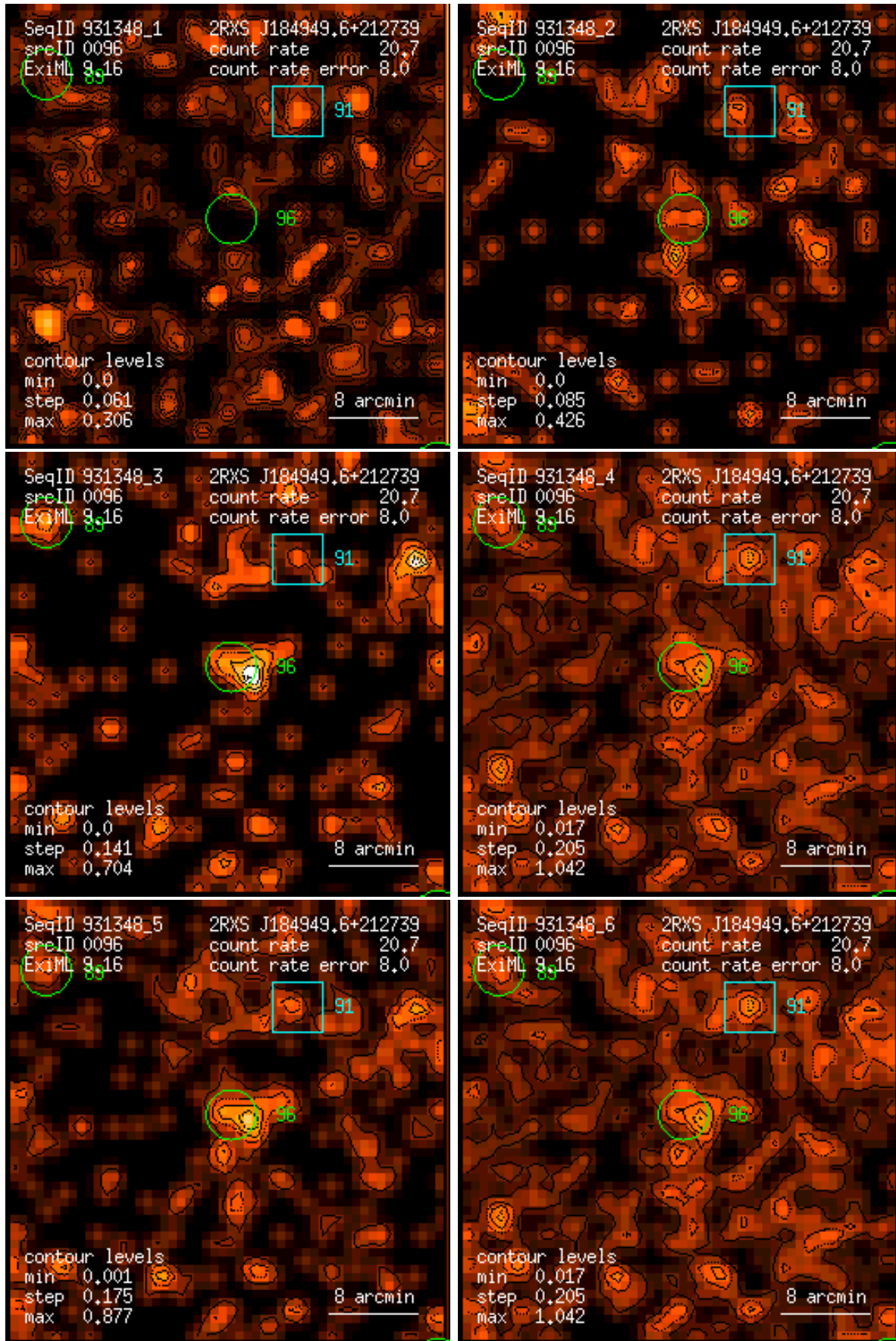
Figure 96: RASS 931348: detection 0096: band rate images, Gaussian filter: (1) PSPC channels 11 – 41, (2) 52 – 90, (3) 91 – 201, (4) 11 – 235, (5) 52 – 201, (6) 11 – 201. Broad band rates in counts/ks. Band rate contour levels in counts/ks/arcmin 2 .
