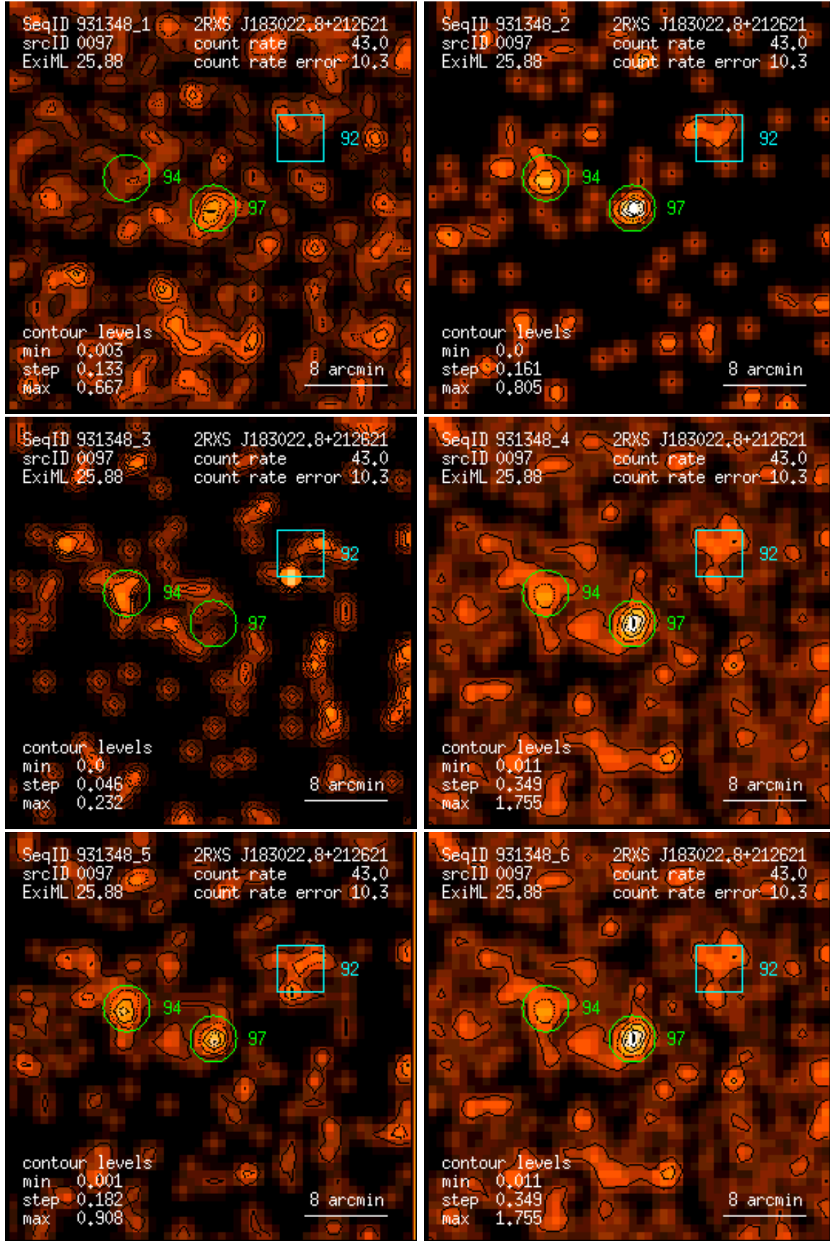
Figure 97: RASS 931348: detection 0097: band rate images, Gaussian filter: (1) PSPC channels 11 – 41, (2) 52 – 90, (3) 91 – 201, (4) 11 – 235, (5) 52 – 201, (6) 11 – 201. Broad band rates in counts/ks. Band rate contour levels in counts/ks/arcmin 2 .
