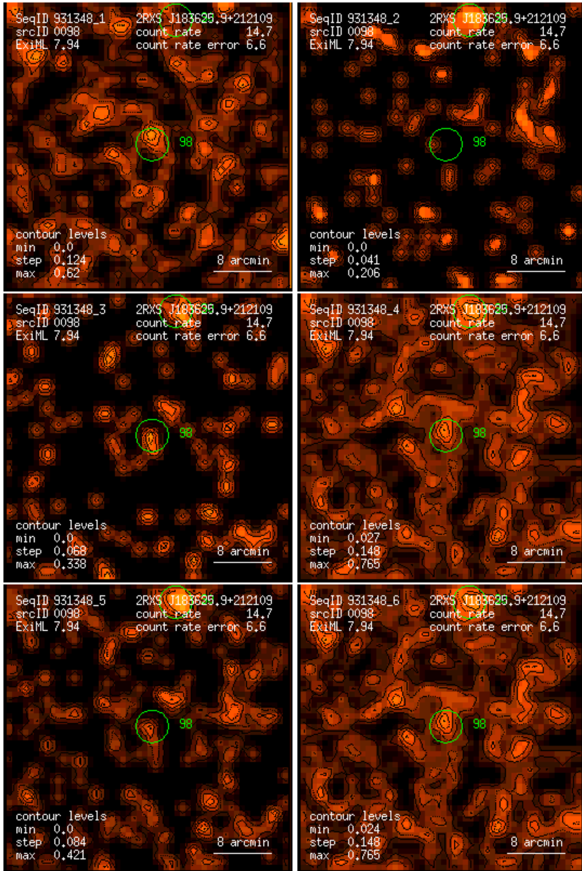
Figure 98: RASS 931348: detection 0098: band rate images, Gaussian filter: (1) PSPC channels 11 – 41, (2) 52 – 90, (3) 91 – 201, (4) 11 – 235, (5) 52 – 201, (6) 11 – 201. Broad band rates in counts/ks. Band rate contour levels in counts/ks/arcmin 2 .
