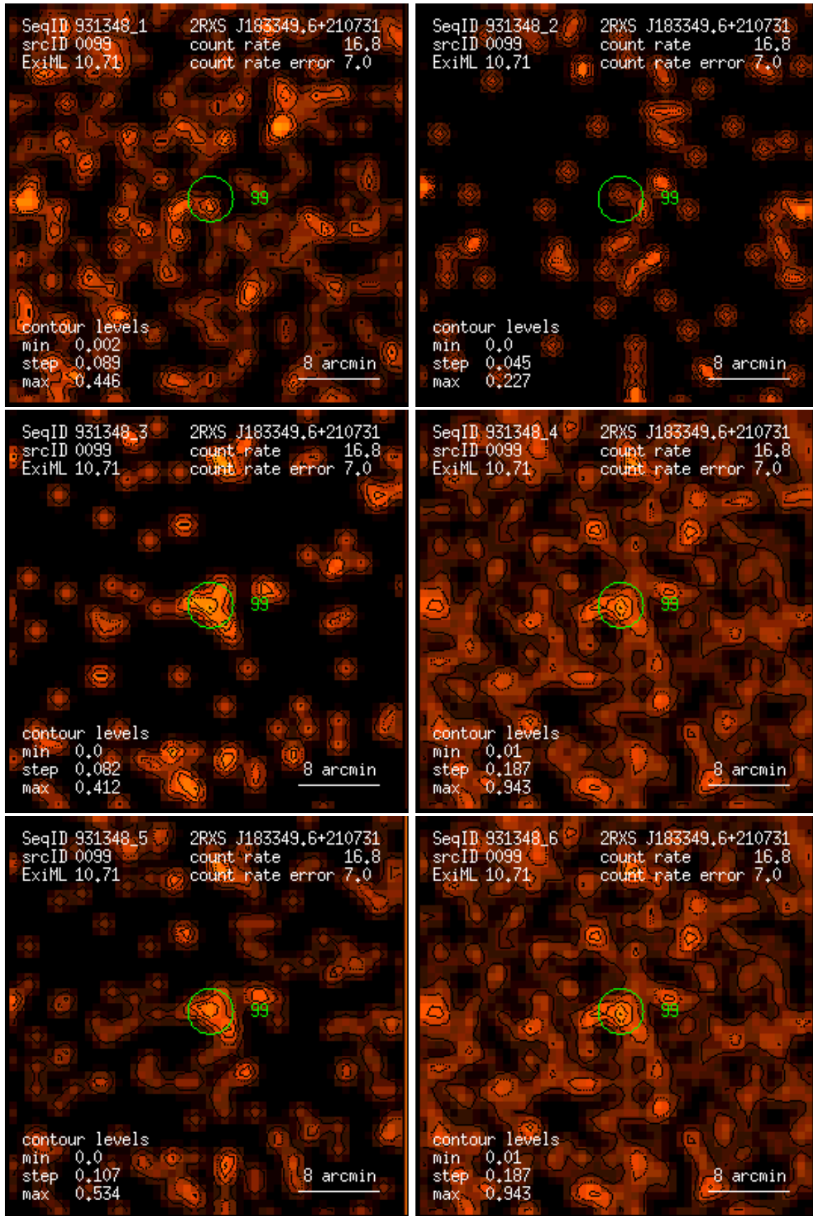
Figure 99: RASS 931348: detection 0099: band rate images, Gaussian filter: (1) PSPC channels 11 – 41, (2) 52 – 90, (3) 91 – 201, (4) 11 – 235, (5) 52 – 201, (6) 11 – 201. Broad band rates in counts/ks. Band rate contour levels in counts/ks/arcmin 2 .
