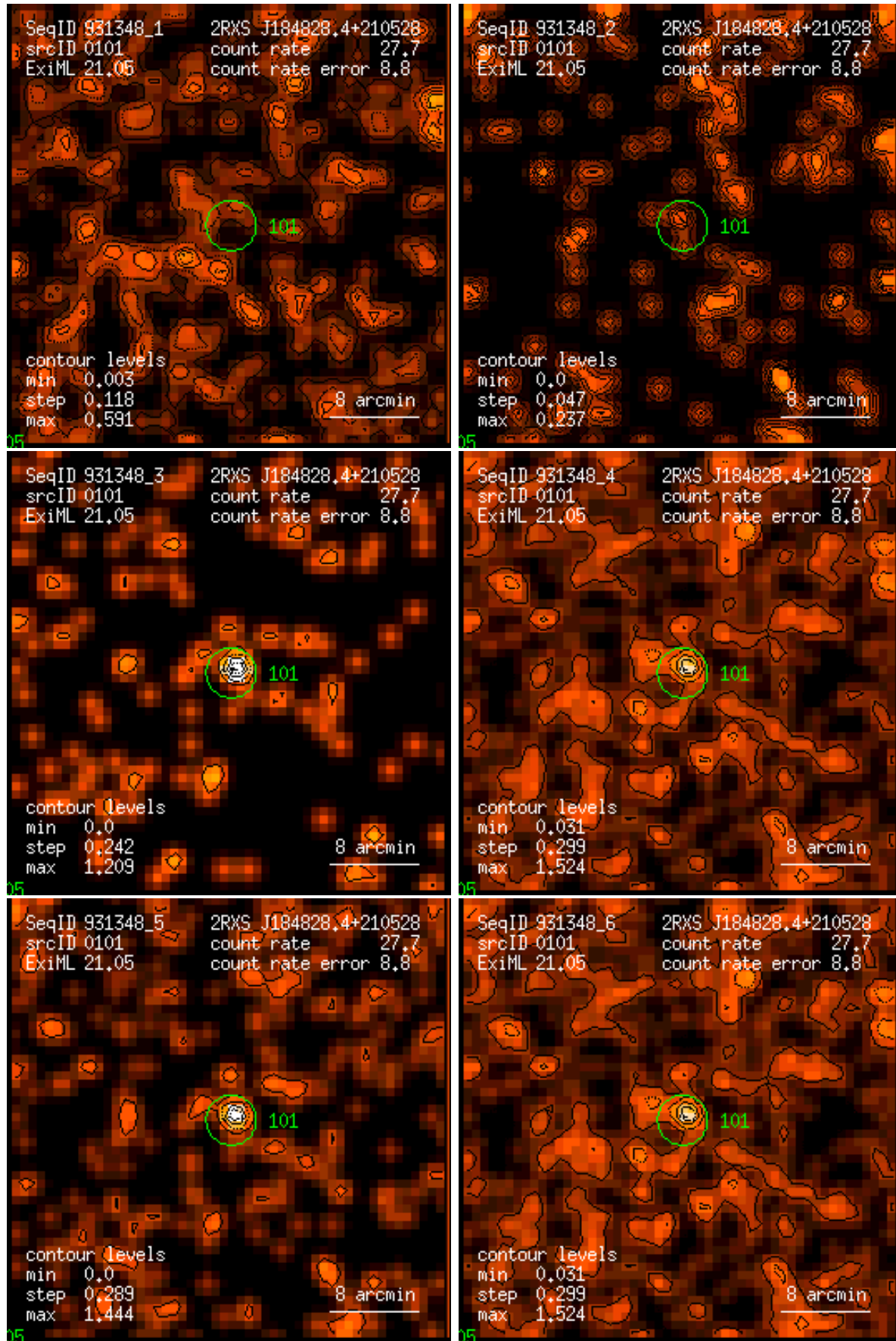
Figure 101: RASS 931348: detection 0101: band rate images, Gaussian filter: (1) PSPC channels 11 – 41, (2) 52 – 90, (3) 91 – 201, (4) 11 – 235, (5) 52 – 201, (6) 11 – 201. Broad band rates in counts/ks. Band rate contour levels in counts/ks/arcmin 2 .
