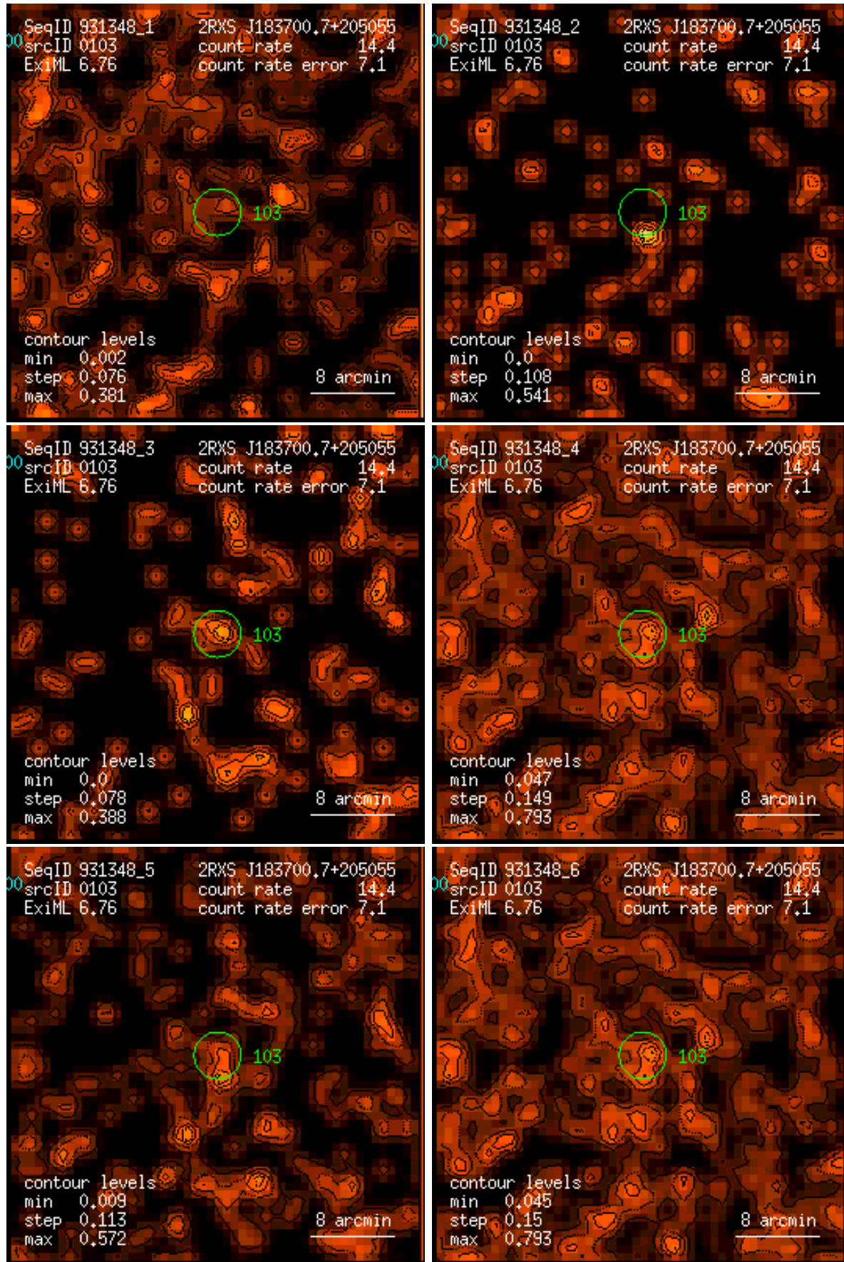
Figure 103: RASS 931348: detection 0103: band rate images, Gaussian filter: (1) PSPC channels 11 – 41, (2) 52 – 90, (3) 91 – 201, (4) 11 – 235, (5) 52 – 201, (6) 11 – 201. Broad band rates in counts/ks. Band rate contour levels in counts/ks/arcmin 2 .
