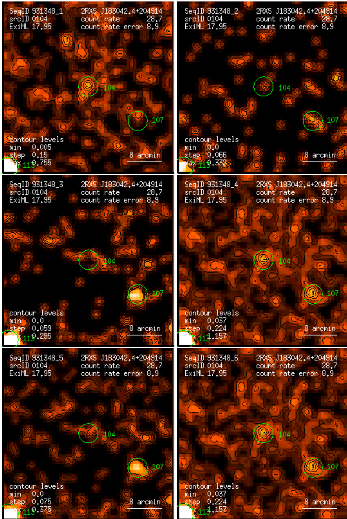
Figure 104: RASS 931348: detection 0104: band rate images, Gaussian filter: (1) PSPC channels 11 – 41, (2) 52 – 90, (3) 91 – 201, (4) 11 – 235, (5) 52 – 201, (6) 11 – 201. Broad band rates in counts/ks. Band rate contour levels in counts/ks/arcmin 2 .
