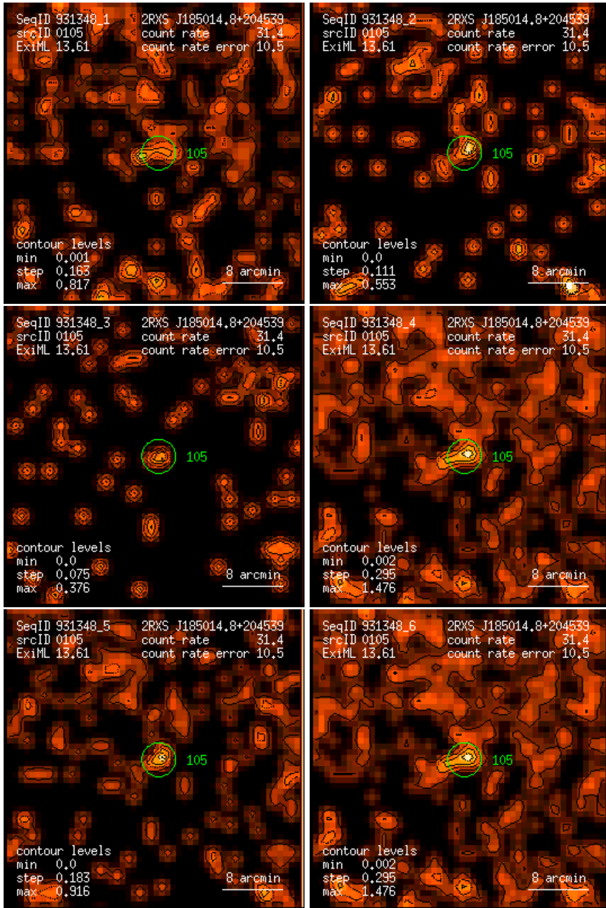
Figure 105: RASS 931348: detection 0105: band rate images, Gaussian filter: (1) PSPC channels 11 – 41, (2) 52 – 90, (3) 91 – 201, (4) 11 – 235, (5) 52 – 201, (6) 11 – 201. Broad band rates in counts/ks. Band rate contour levels in counts/ks/arcmin 2 .
