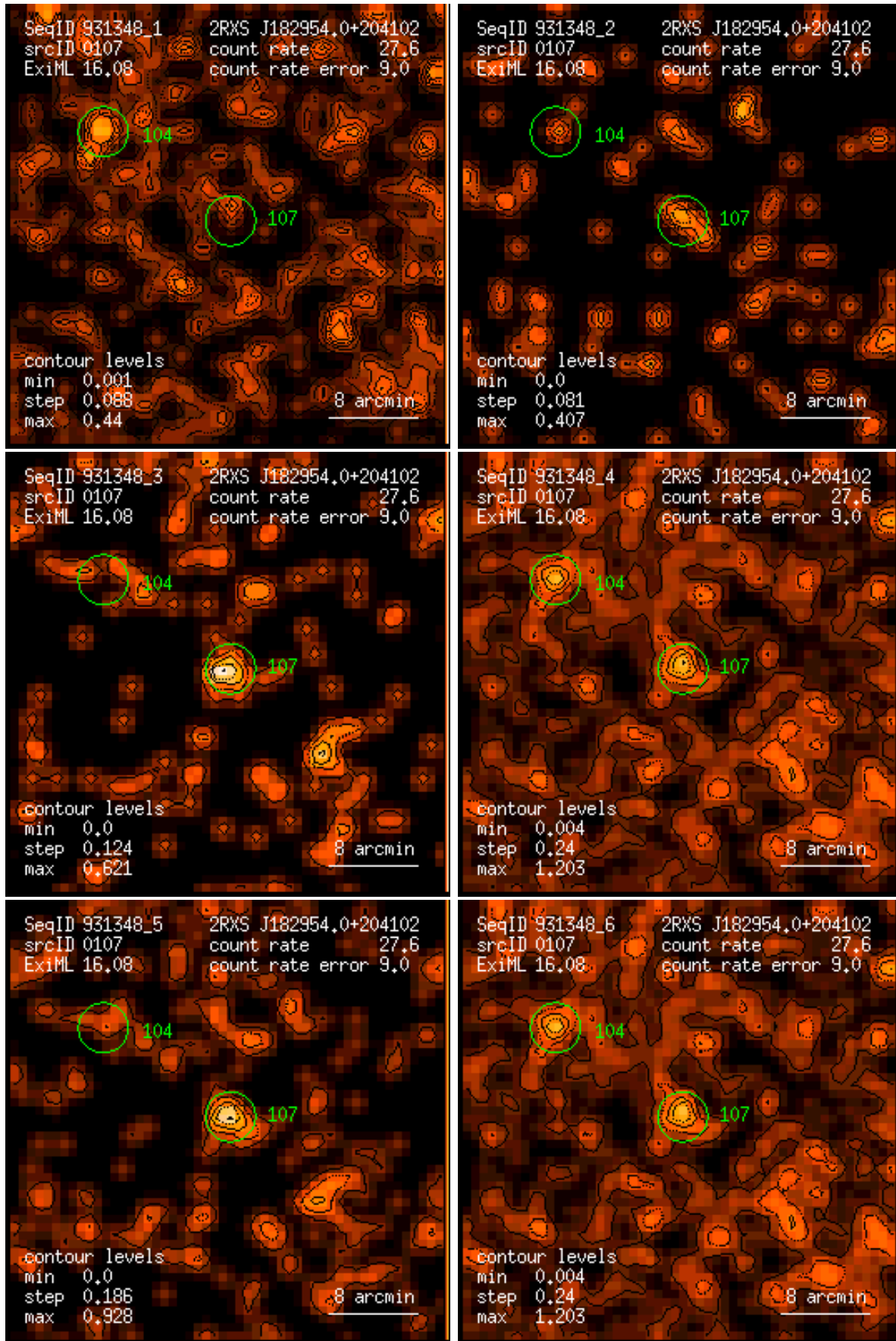
Figure 107: RASS 931348: detection 0107: band rate images, Gaussian filter: (1) PSPC channels 11 – 41, (2) 52 – 90, (3) 91 – 201, (4) 11 – 235, (5) 52 – 201, (6) 11 – 201. Broad band rates in counts/ks. Band rate contour levels in counts/ks/arcmin 2 .
