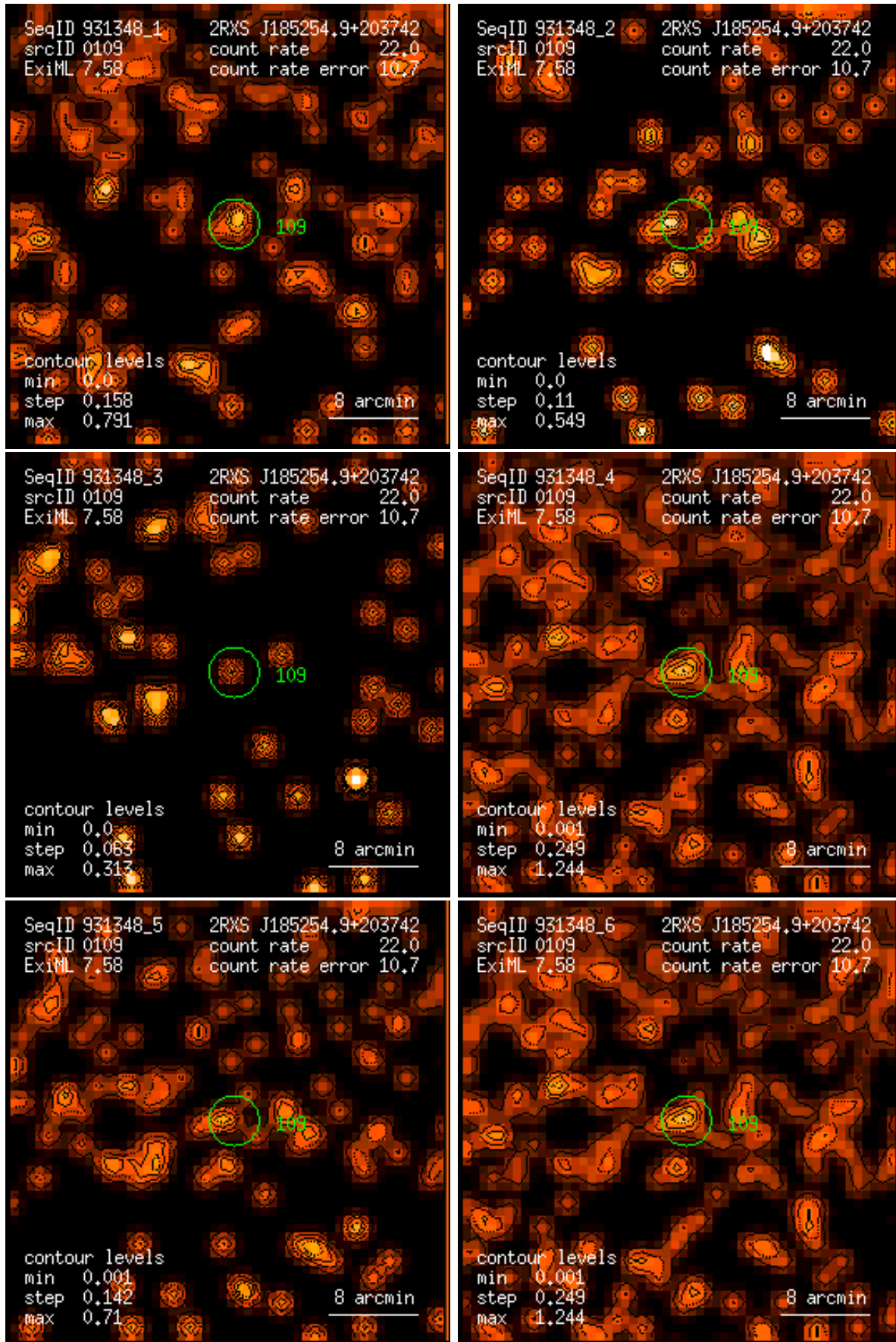
Figure 109: RASS 931348: detection 0109: band rate images, Gaussian filter: (1) PSPC channels 11 – 41, (2) 52 – 90, (3) 91 – 201, (4) 11 – 235, (5) 52 – 201, (6) 11 – 201. Broad band rates in counts/ks. Band rate contour levels in counts/ks/arcmin 2 .
