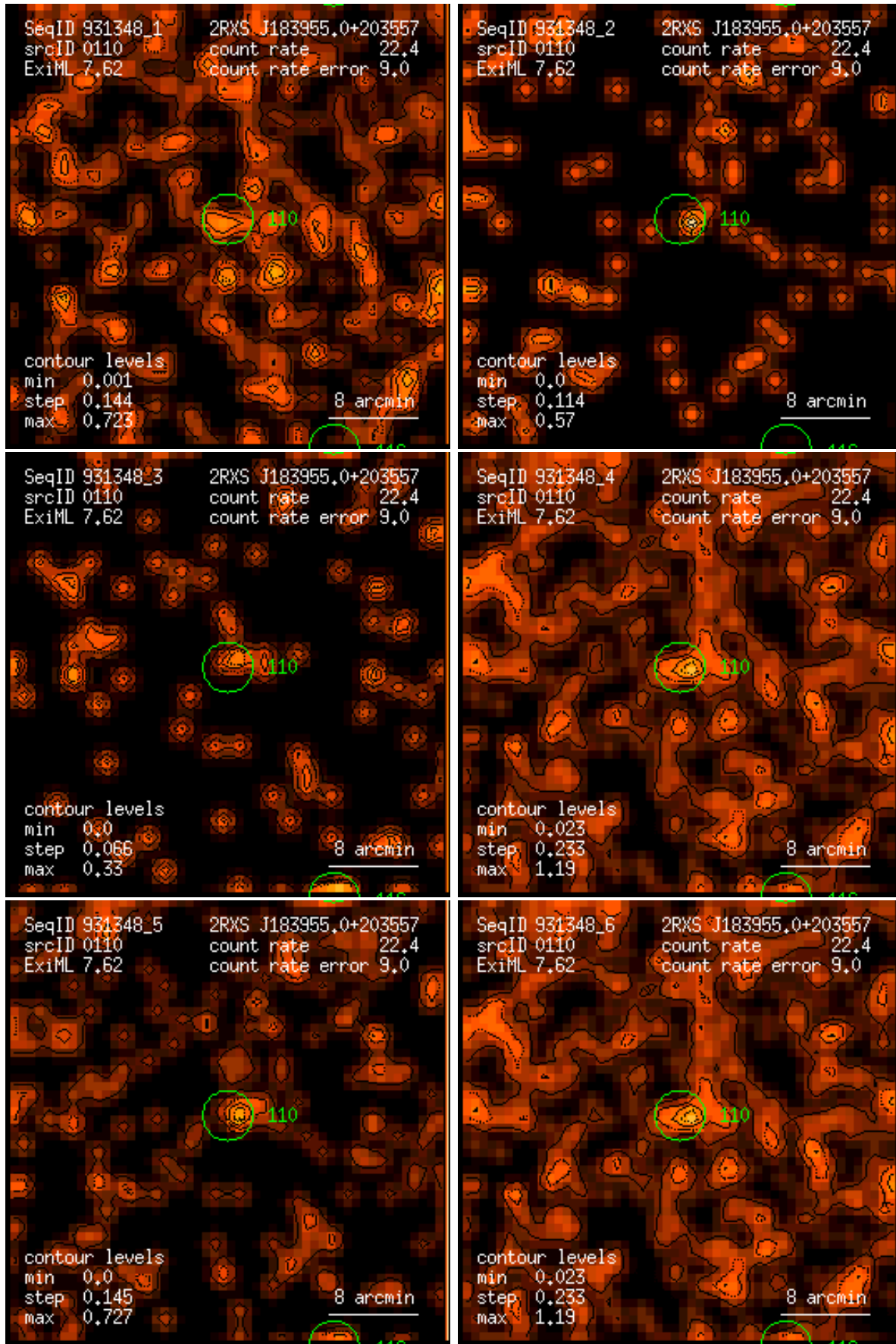
Figure 110: RASS 931348: detection 0110: band rate images, Gaussian filter: (1) PSPC channels 11 – 41, (2) 52 – 90, (3) 91 – 201, (4) 11 – 235, (5) 52 – 201, (6) 11 – 201. Broad band rates in counts/ks. Band rate contour levels in counts/ks/arcmin 2 .
