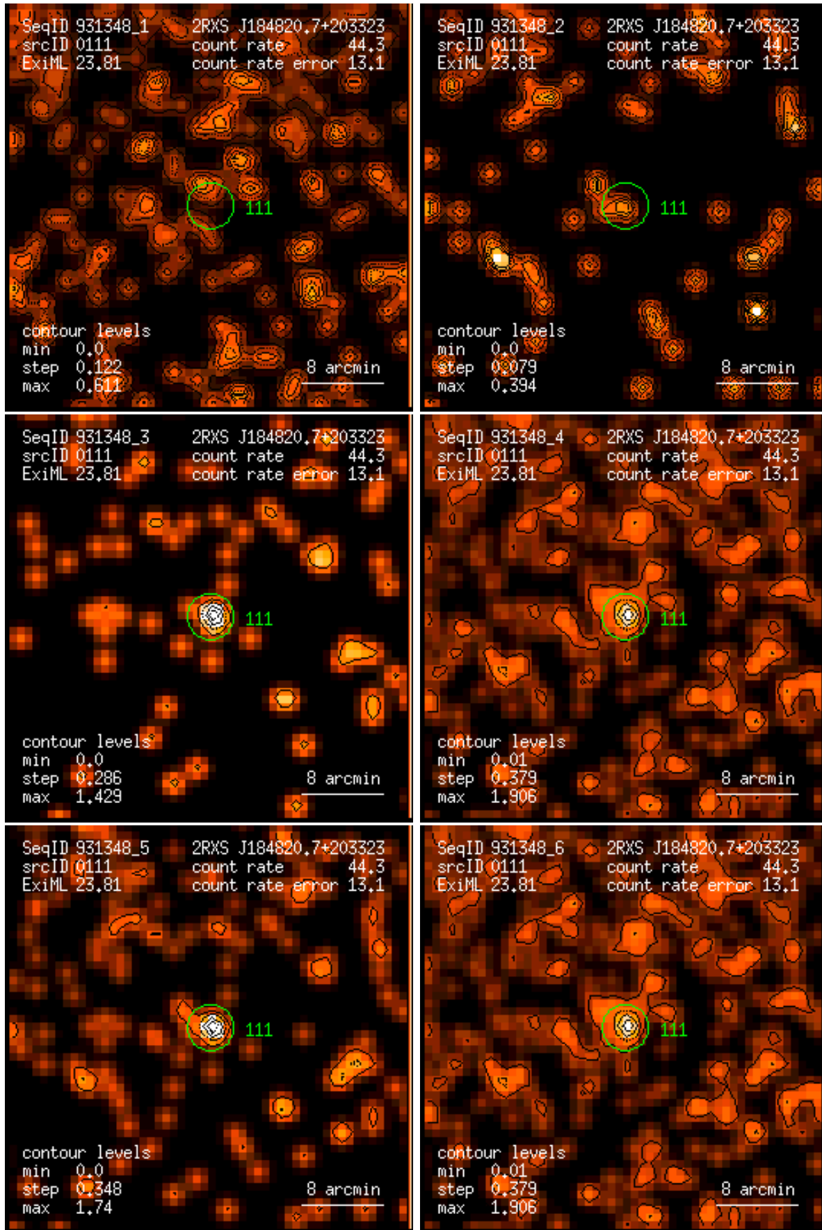
Figure 111: RASS 931348: detection 0111: band rate images, Gaussian filter: (1) PSPC channels 11 – 41, (2) 52 – 90, (3) 91 – 201, (4) 11 – 235, (5) 52 – 201, (6) 11 – 201. Broad band rates in counts/ks. Band rate contour levels in counts/ks/arcmin 2 .
