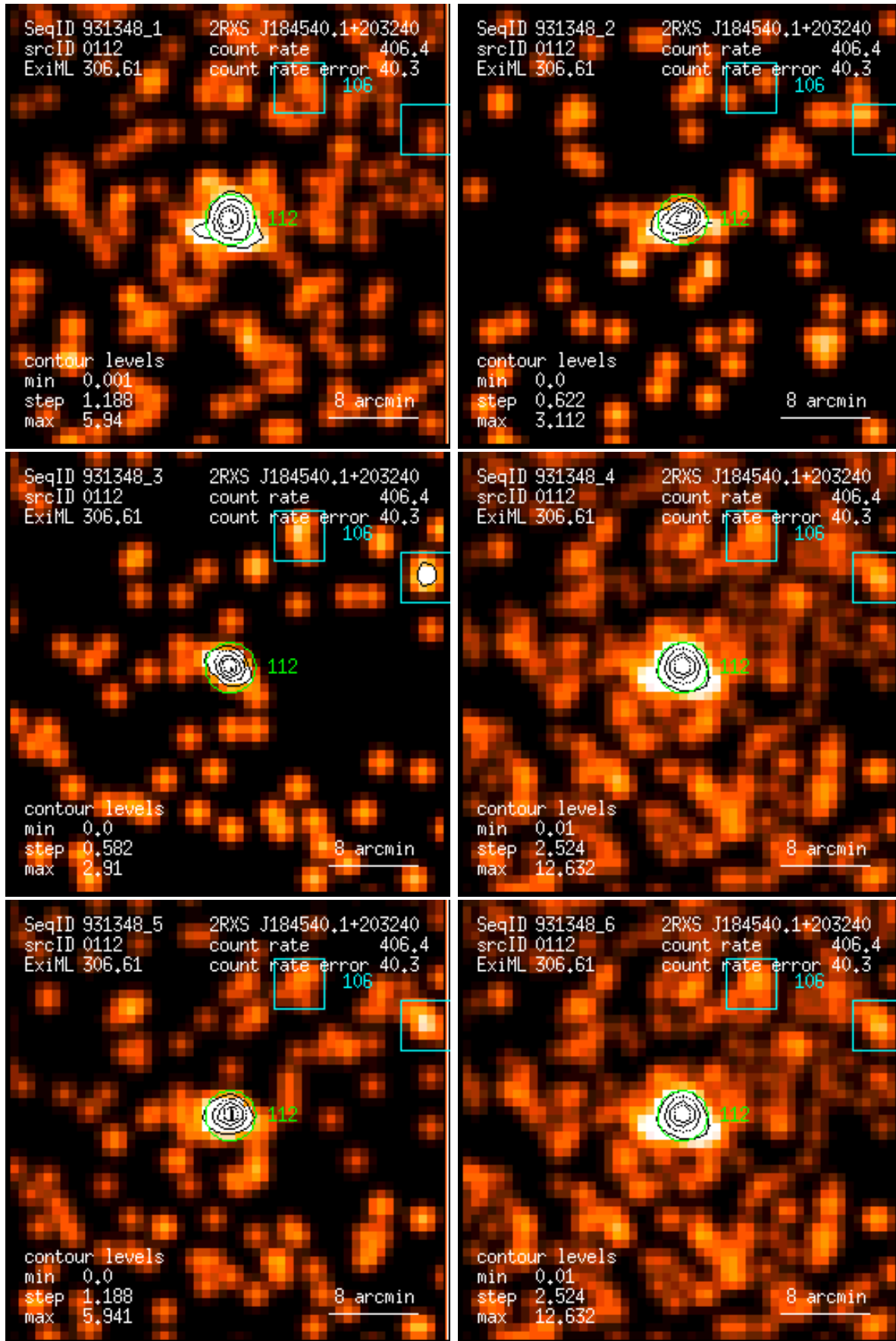
Figure 112: RASS 931348: detection 0112: band rate images, Gaussian filter: (1) PSPC channels 11 – 41, (2) 52 – 90, (3) 91 – 201, (4) 11 – 235, (5) 52 – 201, (6) 11 – 201. Broad band rates in counts/ks. Band rate contour levels in counts/ks/arcmin 2 .
