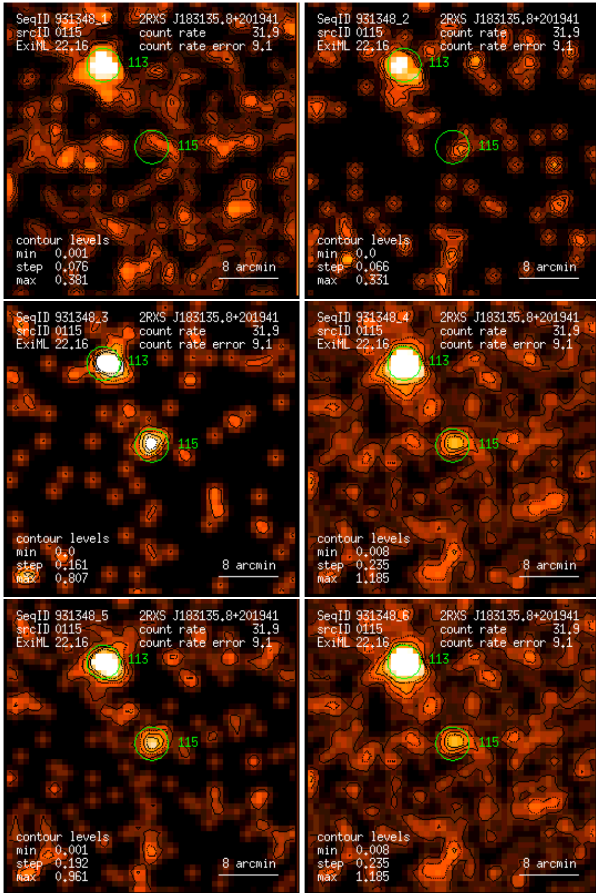
Figure 115: RASS 931348: detection 0115: band rate images, Gaussian filter: (1) PSPC channels 11 – 41, (2) 52 – 90, (3) 91 – 201, (4) 11 – 235, (5) 52 – 201, (6) 11 – 201. Broad band rates in counts/ks. Band rate contour levels in counts/ks/arcmin 2 .
