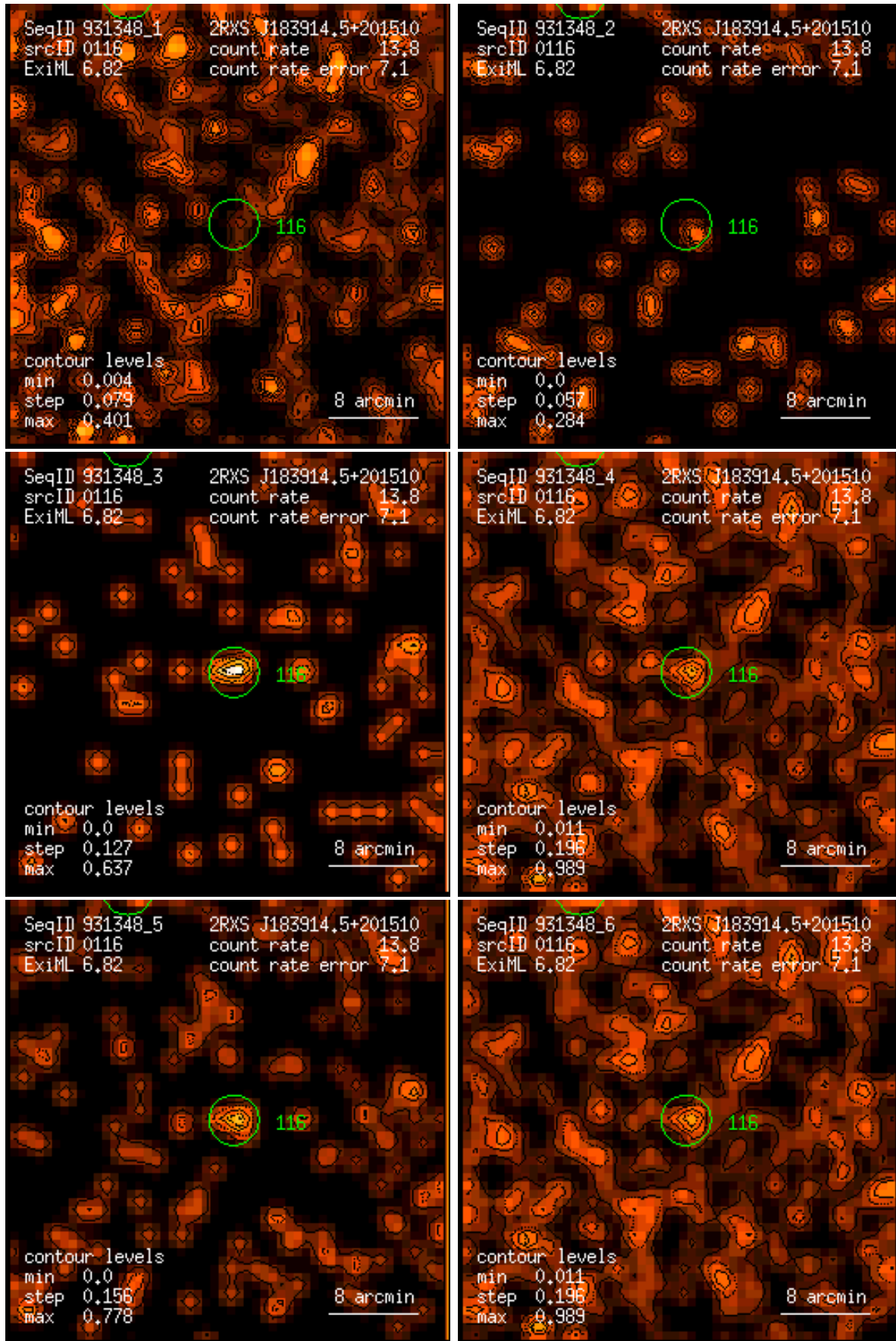
Figure 116: RASS 931348: detection 0116: band rate images, Gaussian filter: (1) PSPC channels 11 – 41, (2) 52 – 90, (3) 91 – 201, (4) 11 – 235, (5) 52 – 201, (6) 11 – 201. Broad band rates in counts/ks. Band rate contour levels in counts/ks/arcmin 2 .
