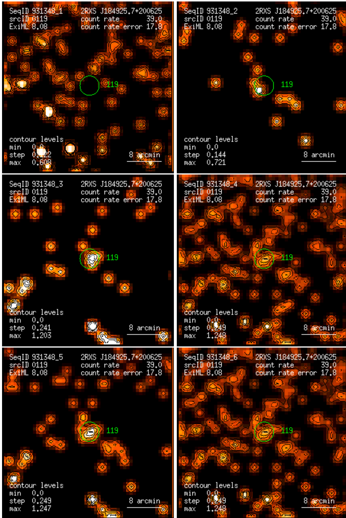
Figure 119: RASS 931348: detection 0119: band rate images, Gaussian filter: (1) PSPC channels 11 – 41, (2) 52 – 90, (3) 91 – 201, (4) 11 – 235, (5) 52 – 201, (6) 11 – 201. Broad band rates in counts/ks. Band rate contour levels in counts/ks/arcmin 2 .
