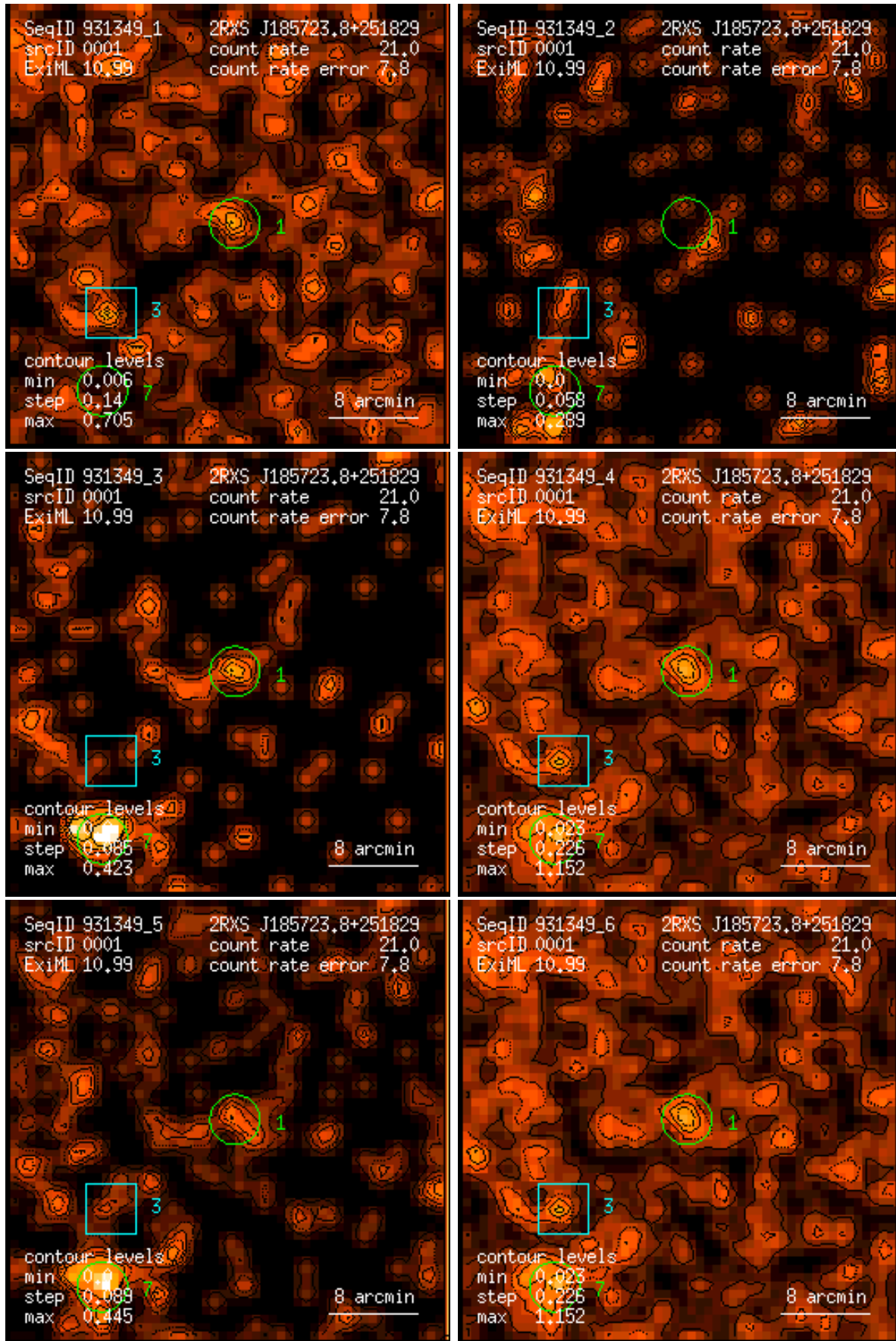
Figure 1: RASS 931349: detection 0001: band rate images, Gaussian filter: (1) PSPC channels 11 – 41, (2) 52 – 90, (3) 91 – 201, (4) 11 – 235, (5) 52 – 201, (6) 11 – 201. Broad band rates in counts/ks. Band rate contour levels in counts/ks/arcmin 2 .
