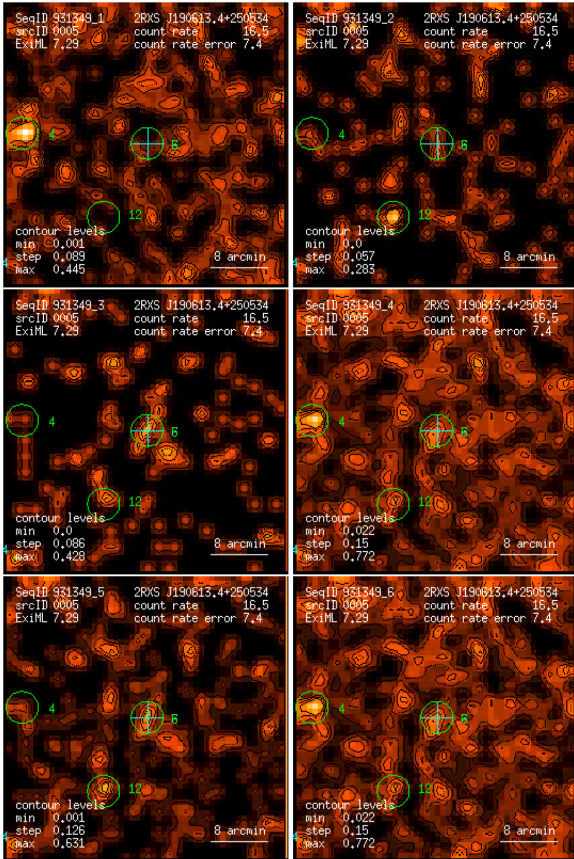
Figure 5: RASS 931349: detection 0005: band rate images, Gaussian filter: (1) PSPC channels 11 – 41, (2) 52 – 90, (3) 91 – 201, (4) 11 – 235, (5) 52 – 201, (6) 11 – 201. Broad band rates in counts/ks. Band rate contour levels in counts/ks/arcmin 2 .
