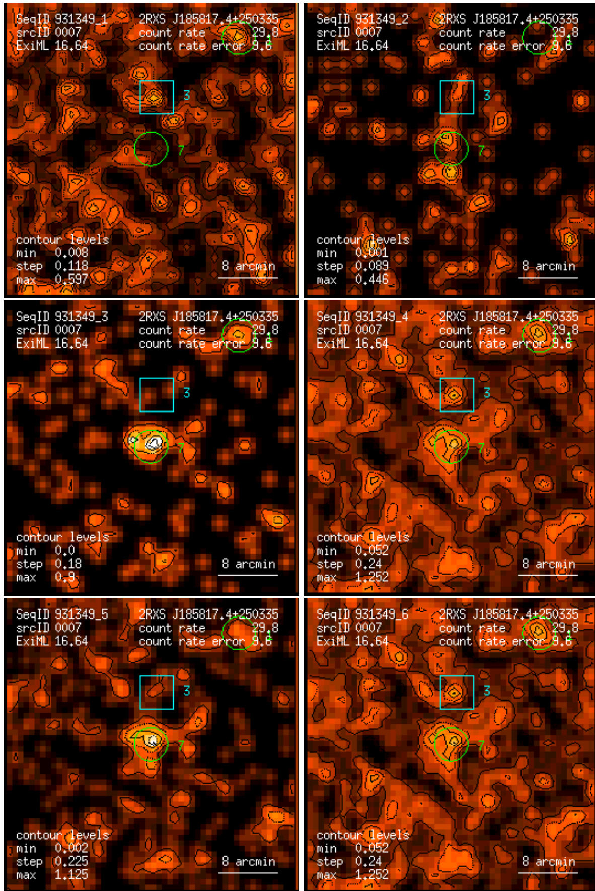
Figure 7: RASS 931349: detection 0007: band rate images, Gaussian filter: (1) PSPC channels 11 – 41, (2) 52 – 90, (3) 91 – 201, (4) 11 – 235, (5) 52 – 201, (6) 11 – 201. Broad band rates in counts/ks. Band rate contour levels in counts/ks/arcmin 2 .
