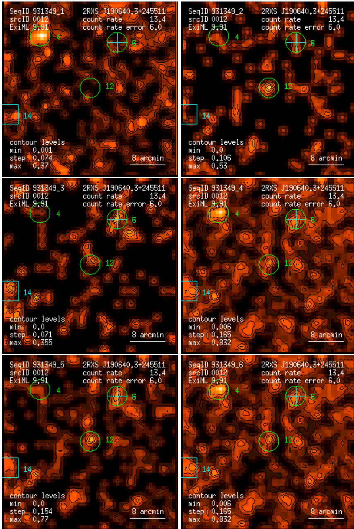
Figure 12: RASS 931349: detection 0012: band rate images, Gaussian filter: (1) PSPC channels 11 – 41, (2) 52 – 90, (3) 91 – 201, (4) 11 – 235, (5) 52 – 201, (6) 11 – 201. Broad band rates in counts/ks. Band rate contour levels in counts/ks/arcmin 2 .
