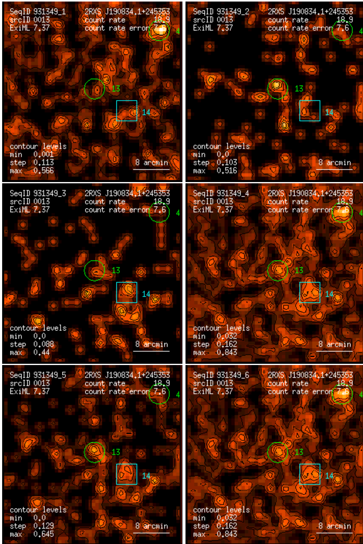
Figure 13: RASS 931349: detection 0013: band rate images, Gaussian filter: (1) PSPC channels 11 – 41, (2) 52 – 90, (3) 91 – 201, (4) 11 – 235, (5) 52 – 201, (6) 11 – 201. Broad band rates in counts/ks. Band rate contour levels in counts/ks/arcmin 2 .
