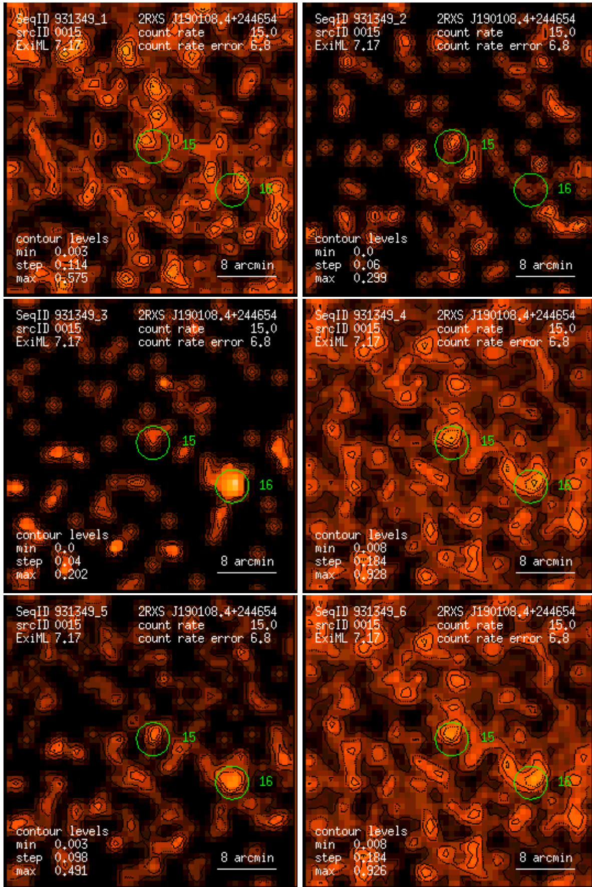
Figure 15: RASS 931349: detection 0015: band rate images, Gaussian filter: (1) PSPC channels 11 – 41, (2) 52 – 90, (3) 91 – 201, (4) 11 – 235, (5) 52 – 201, (6) 11 – 201. Broad band rates in counts/ks. Band rate contour levels in counts/ks/arcmin 2 .
