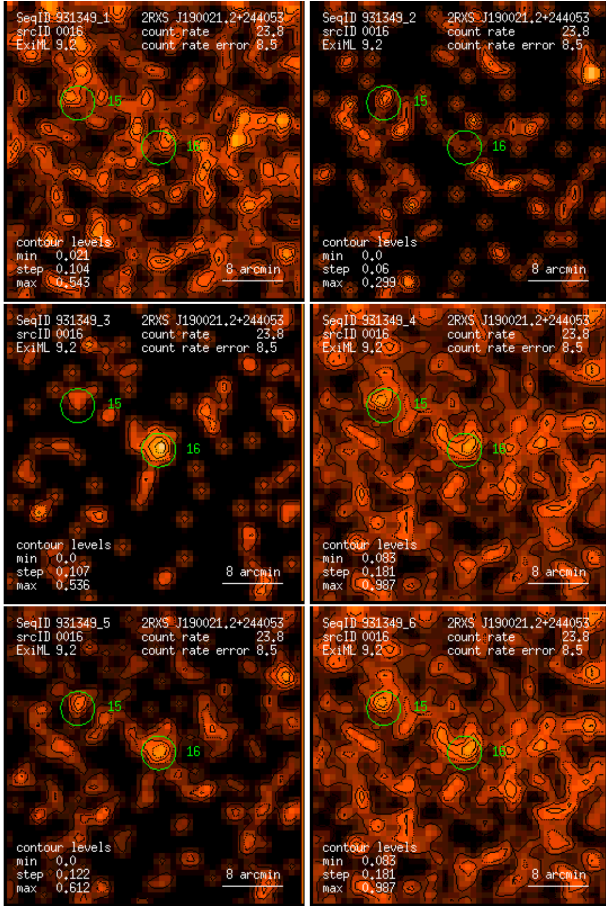
Figure 16: RASS 931349: detection 0016: band rate images, Gaussian filter: (1) PSPC channels 11 – 41, (2) 52 – 90, (3) 91 – 201, (4) 11 – 235, (5) 52 – 201, (6) 11 – 201. Broad band rates in counts/ks. Band rate contour levels in counts/ks/arcmin 2 .
