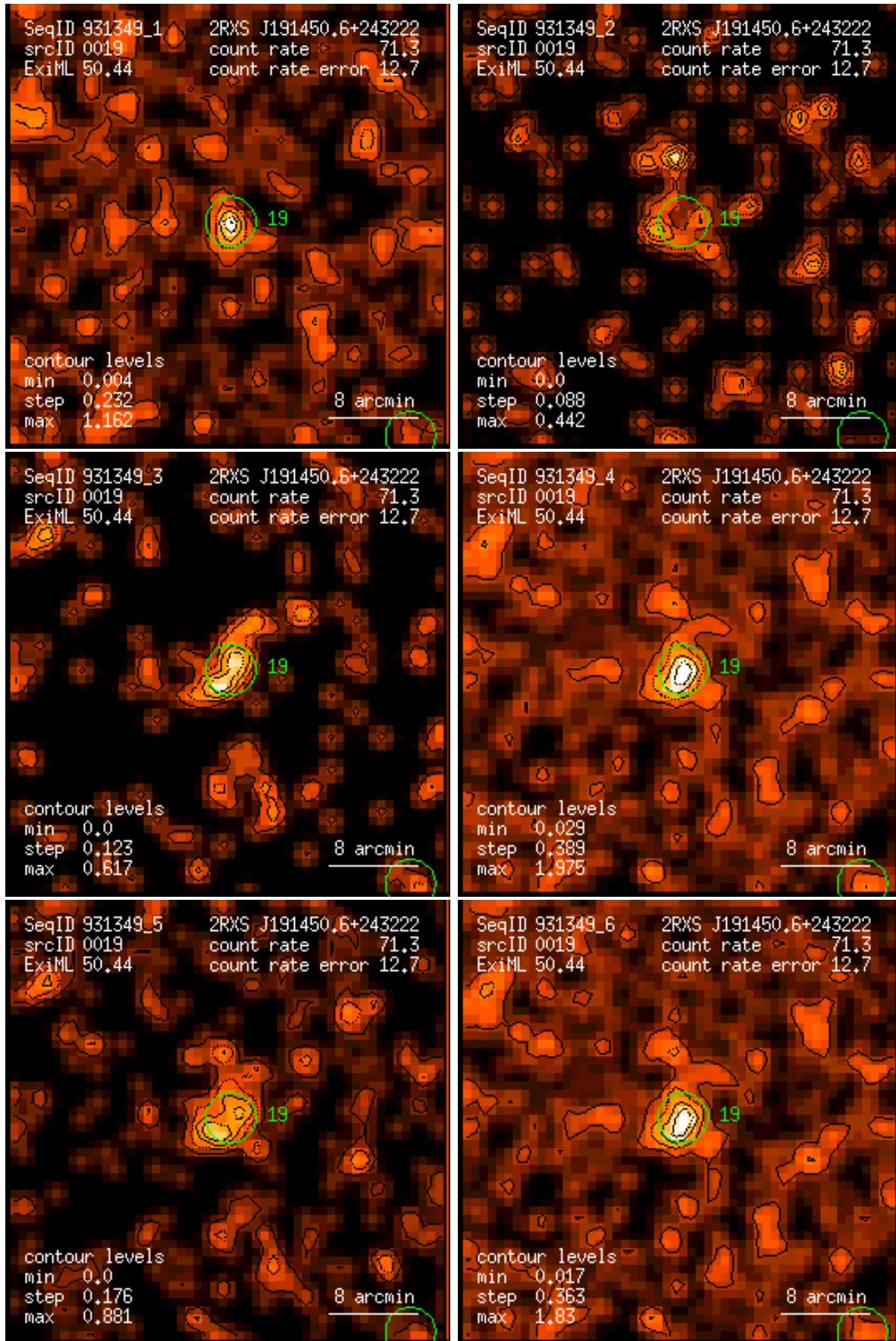
Figure 19: RASS 931349: detection 0019: band rate images, Gaussian filter: (1) PSPC channels 11 – 41, (2) 52 – 90, (3) 91 – 201, (4) 11 – 235, (5) 52 – 201, (6) 11 – 201. Broad band rates in counts/ks. Band rate contour levels in counts/ks/arcmin 2 .
