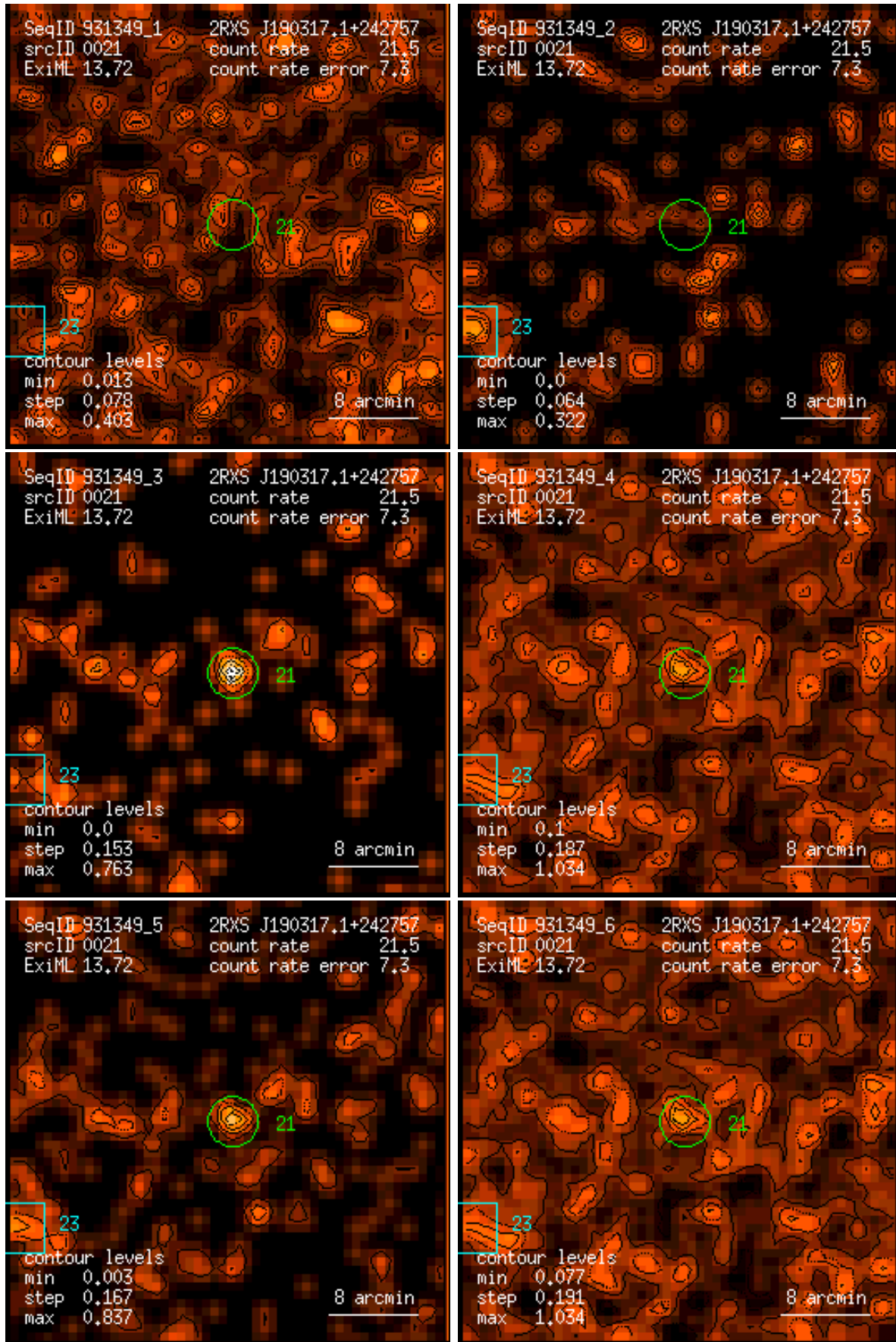
Figure 21: RASS 931349: detection 0021: band rate images, Gaussian filter: (1) PSPC channels 11 – 41, (2) 52 – 90, (3) 91 – 201, (4) 11 – 235, (5) 52 – 201, (6) 11 – 201. Broad band rates in counts/ks. Band rate contour levels in counts/ks/arcmin 2 .
