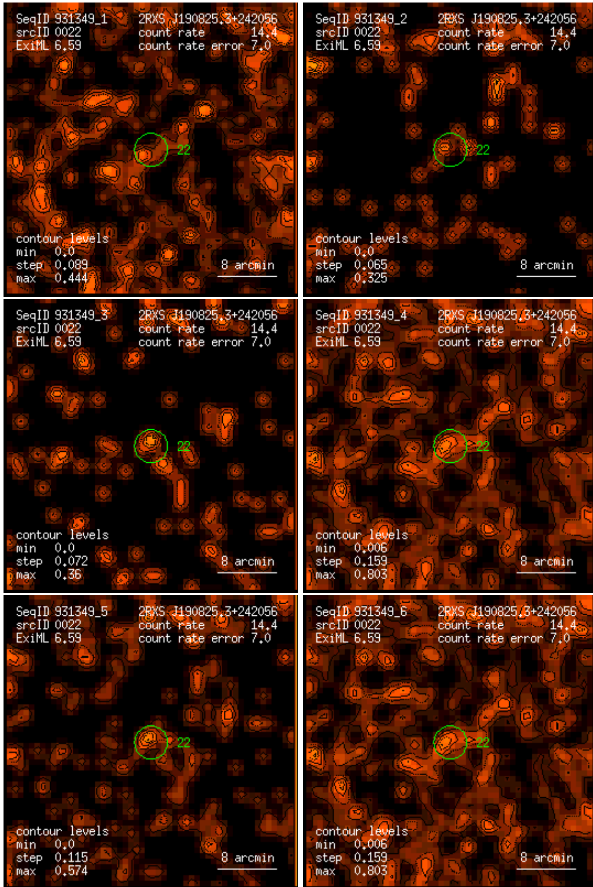
Figure 22: RASS 931349: detection 0022: band rate images, Gaussian filter: (1) PSPC channels 11 – 41, (2) 52 – 90, (3) 91 – 201, (4) 11 – 235, (5) 52 – 201, (6) 11 – 201. Broad band rates in counts/ks. Band rate contour levels in counts/ks/arcmin 2 .
