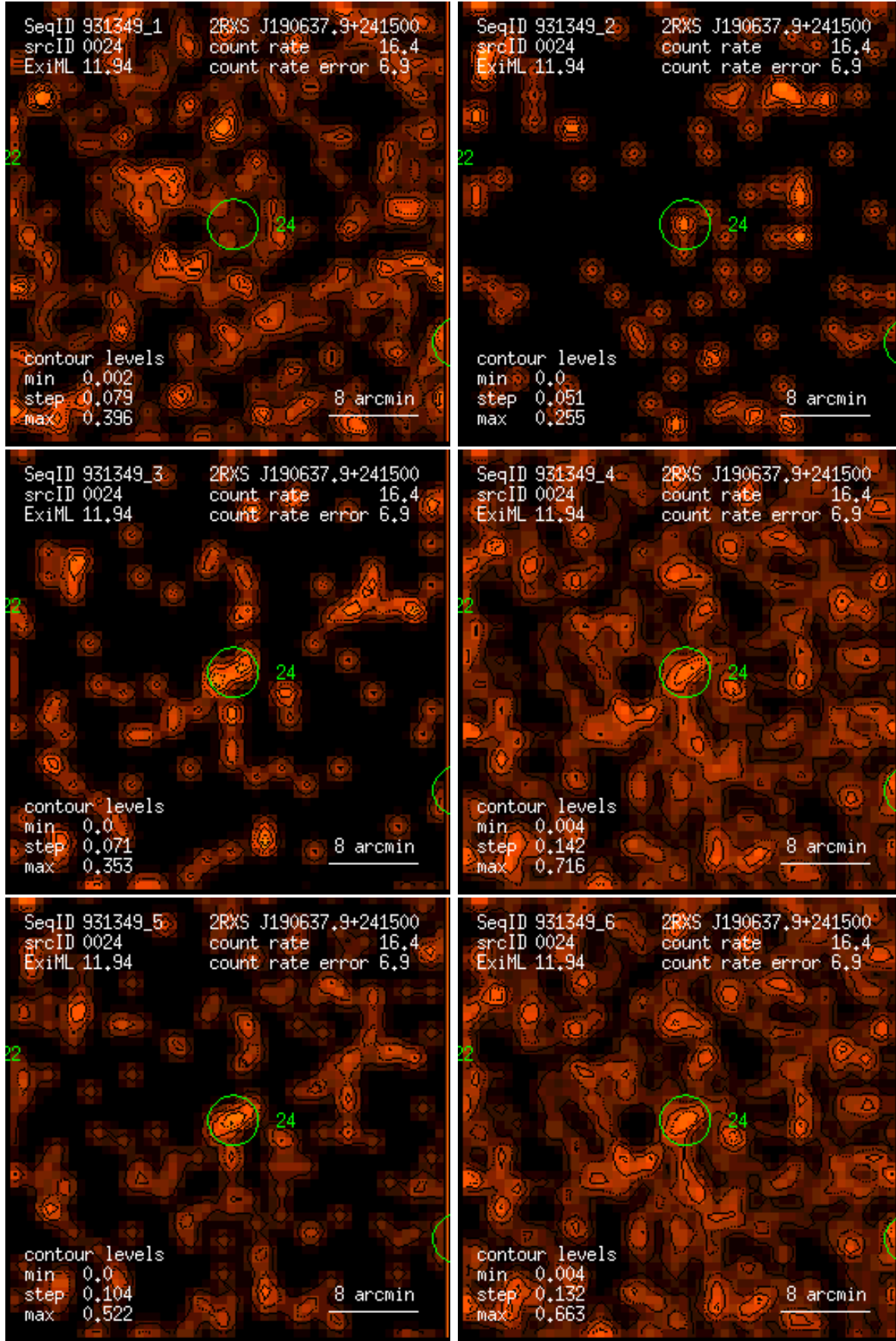
Figure 24: RASS 931349: detection 0024: band rate images, Gaussian filter: (1) PSPC channels 11 – 41, (2) 52 – 90, (3) 91 – 201, (4) 11 – 235, (5) 52 – 201, (6) 11 – 201. Broad band rates in counts/ks. Band rate contour levels in counts/ks/arcmin 2 .
