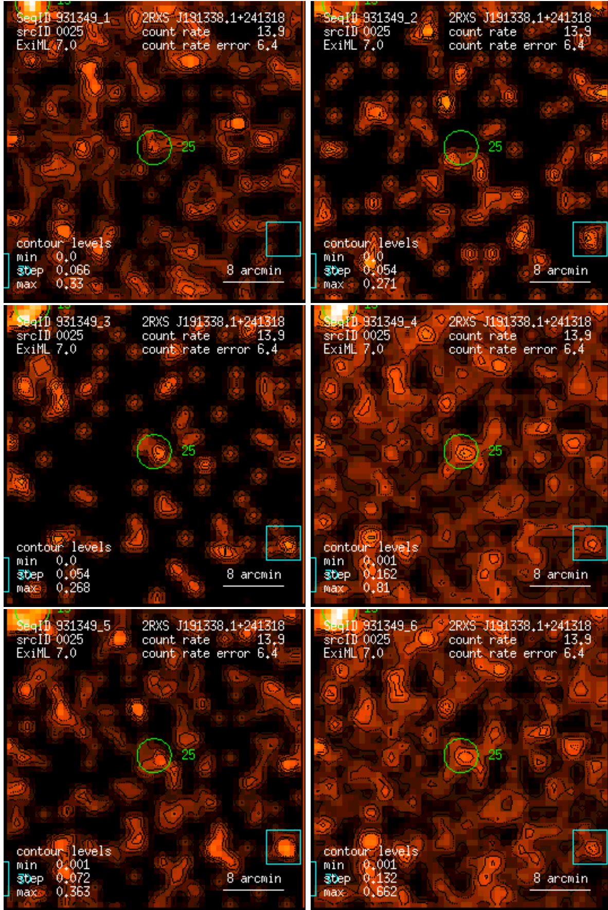
Figure 25: RASS 931349: detection 0025: band rate images, Gaussian filter: (1) PSPC channels 11 – 41, (2) 52 – 90, (3) 91 – 201, (4) 11 – 235, (5) 52 – 201, (6) 11 – 201. Broad band rates in counts/ks. Band rate contour levels in counts/ks/arcmin 2 .
