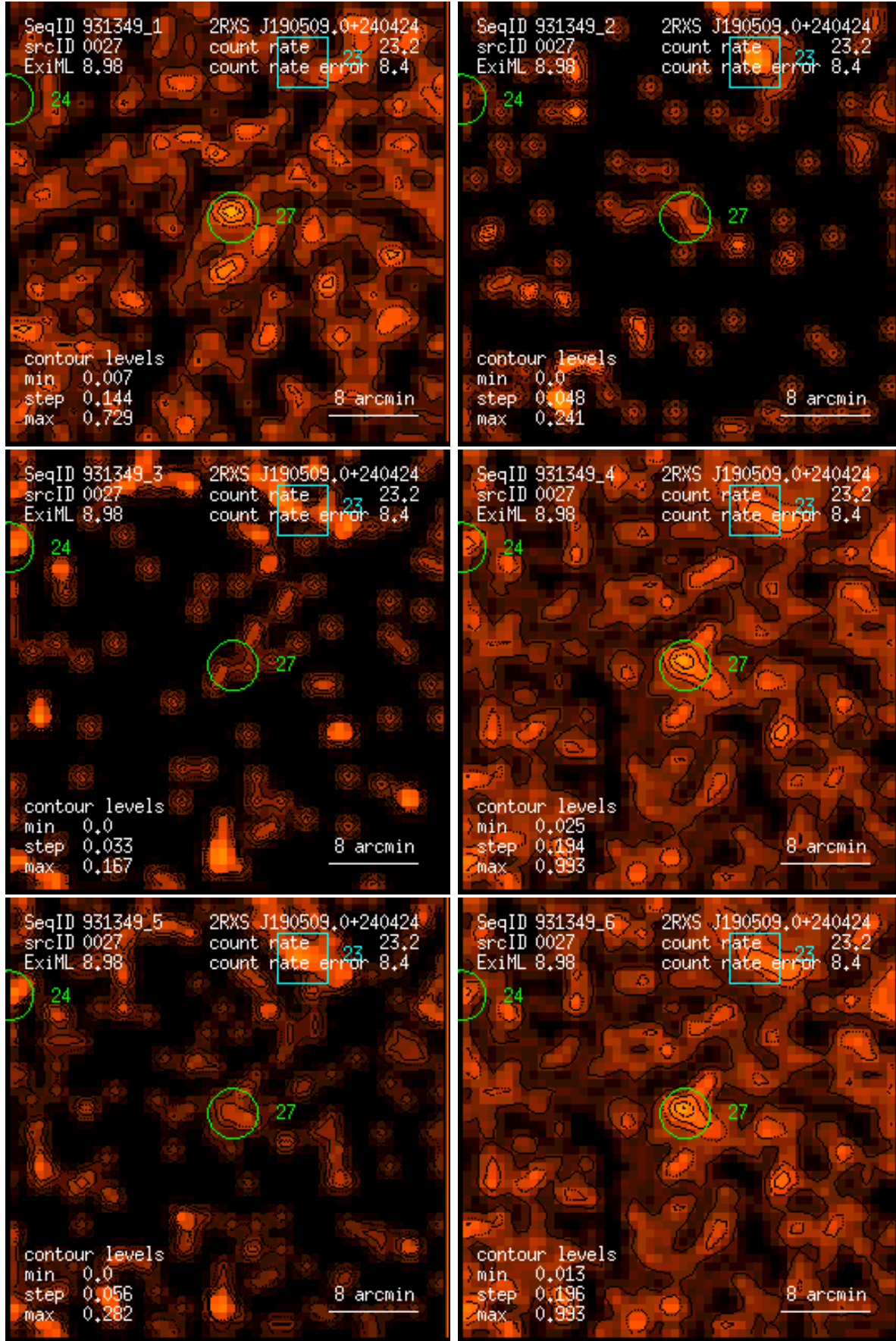
Figure 27: RASS 931349: detection 0027: band rate images, Gaussian filter: (1) PSPC channels 11 – 41, (2) 52 – 90, (3) 91 – 201, (4) 11 – 235, (5) 52 – 201, (6) 11 – 201. Broad band rates in counts/ks. Band rate contour levels in counts/ks/arcmin 2 .
