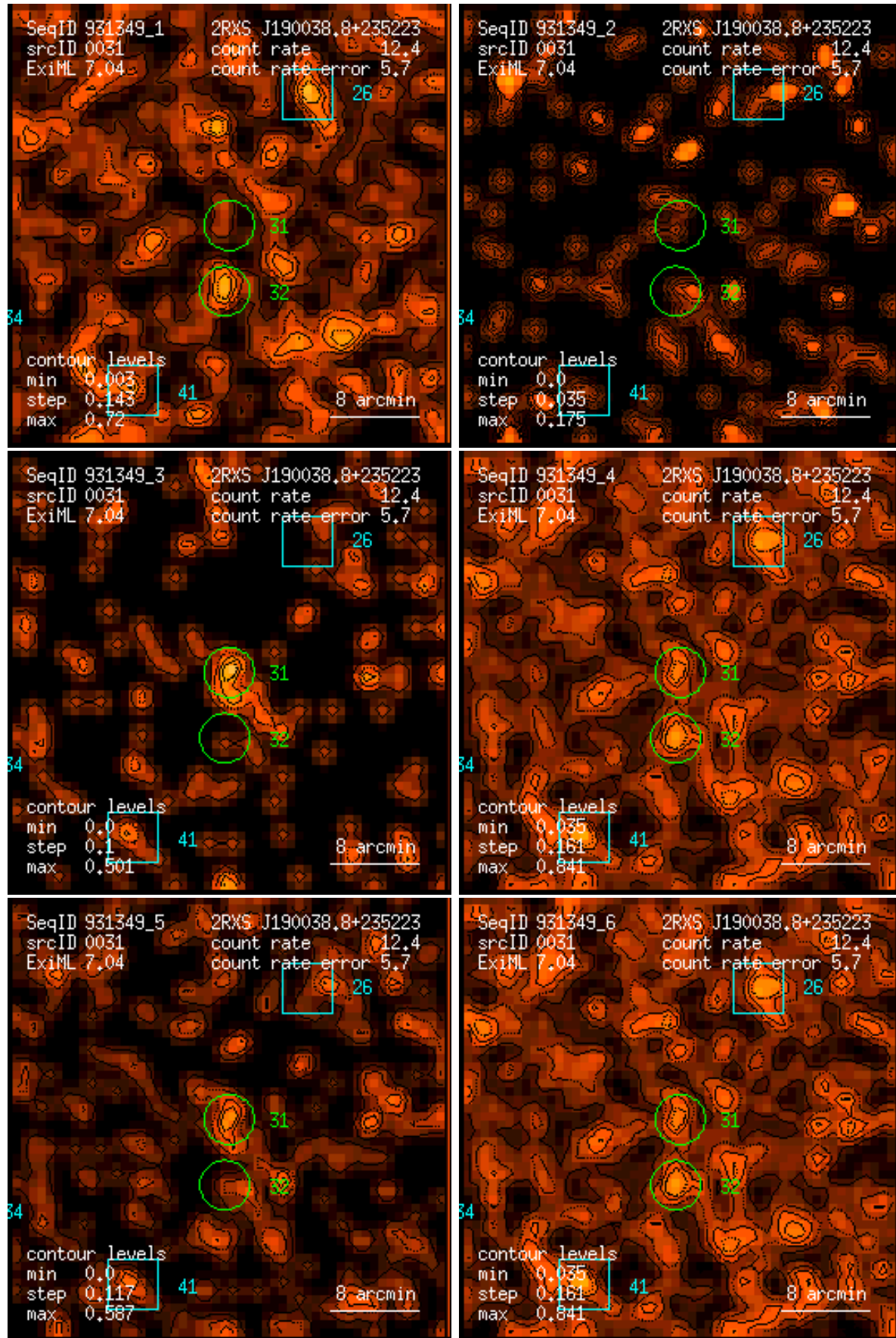
Figure 31: RASS 931349: detection 0031: band rate images, Gaussian filter: (1) PSPC channels 11 – 41, (2) 52 – 90, (3) 91 – 201, (4) 11 – 235, (5) 52 – 201, (6) 11 – 201. Broad band rates in counts/ks. Band rate contour levels in counts/ks/arcmin 2 .
