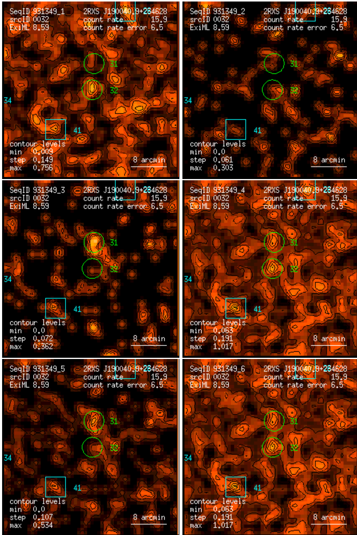
Figure 32: RASS 931349: detection 0032: band rate images, Gaussian filter: (1) PSPC channels 11 – 41, (2) 52 – 90, (3) 91 – 201, (4) 11 – 235, (5) 52 – 201, (6) 11 – 201. Broad band rates in counts/ks. Band rate contour levels in counts/ks/arcmin 2 .
