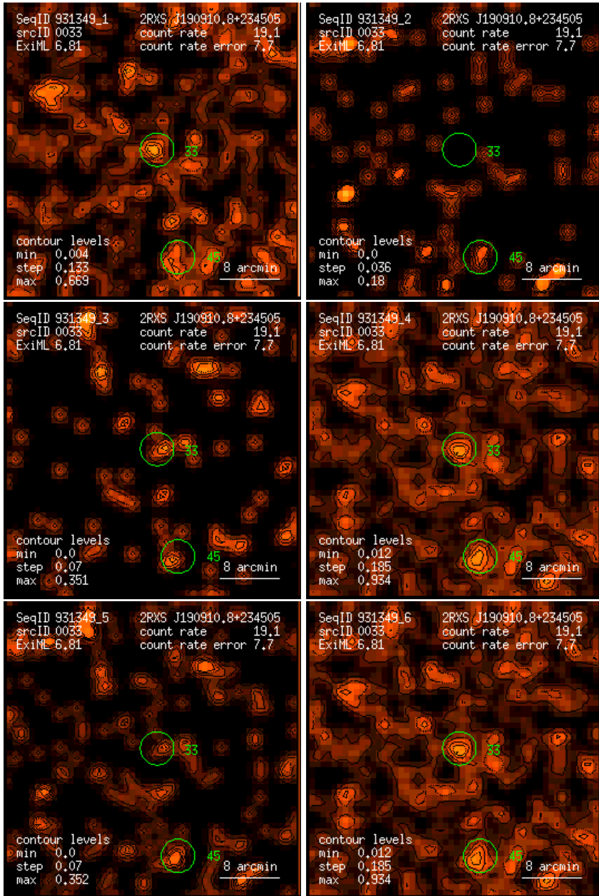
Figure 33: RASS 931349: detection 0033: band rate images, Gaussian filter: (1) PSPC channels 11 – 41, (2) 52 – 90, (3) 91 – 201, (4) 11 – 235, (5) 52 – 201, (6) 11 – 201. Broad band rates in counts/ks. Band rate contour levels in counts/ks/arcmin 2 .
