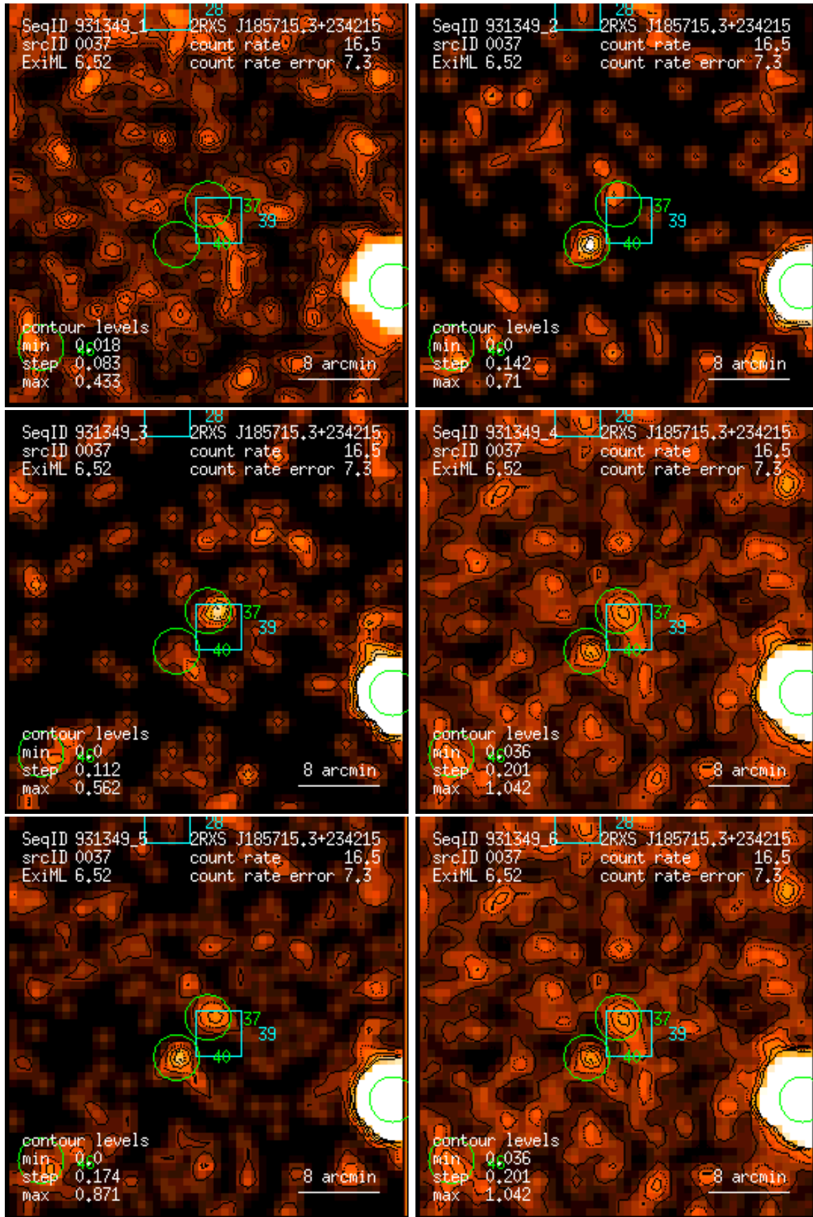
Figure 37: RASS 931349: detection 0037: band rate images, Gaussian filter: (1) PSPC channels 11 – 41, (2) 52 – 90, (3) 91 – 201, (4) 11 – 235, (5) 52 – 201, (6) 11 – 201. Broad band rates in counts/ks. Band rate contour levels in counts/ks/arcmin 2 .
