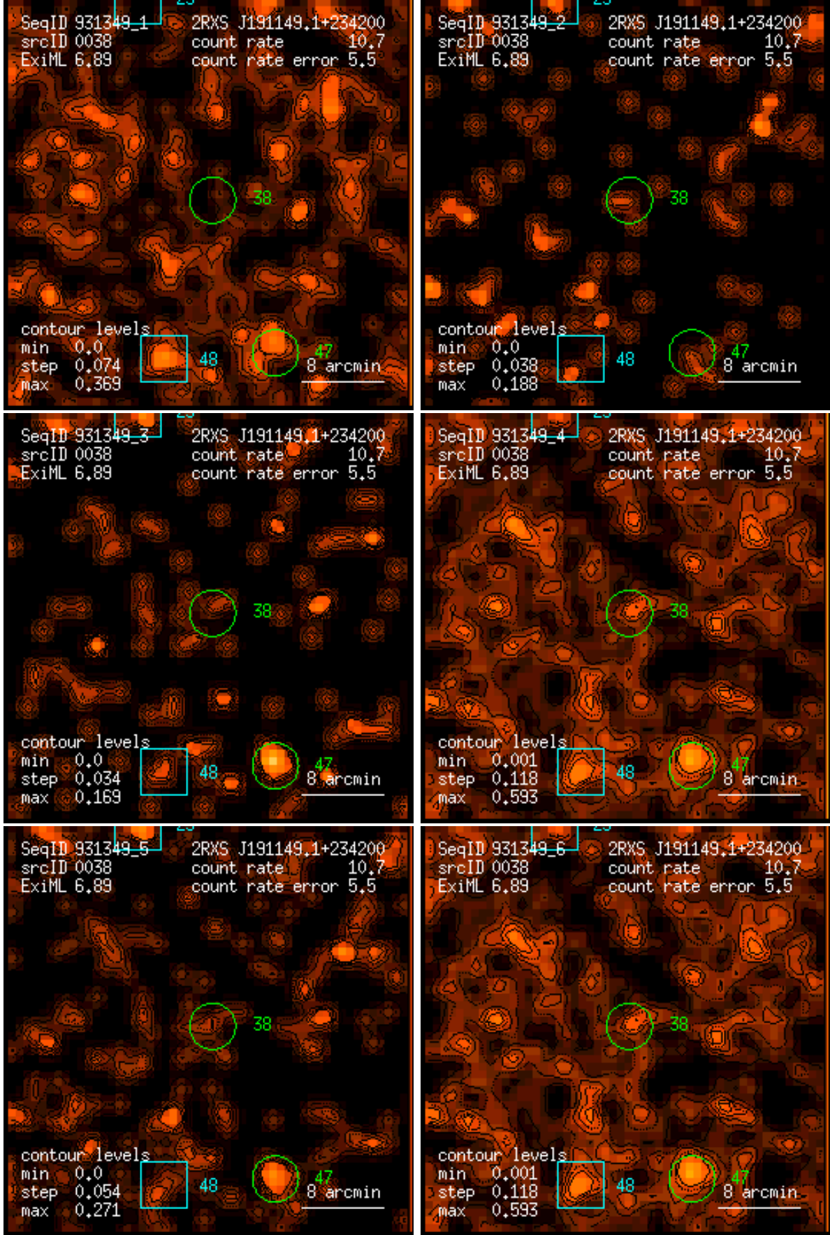
Figure 38: RASS 931349: detection 0038: band rate images, Gaussian filter: (1) PSPC channels 11 – 41, (2) 52 – 90, (3) 91 – 201, (4) 11 – 235, (5) 52 – 201, (6) 11 – 201. Broad band rates in counts/ks. Band rate contour levels in counts/ks/arcmin 2 .
