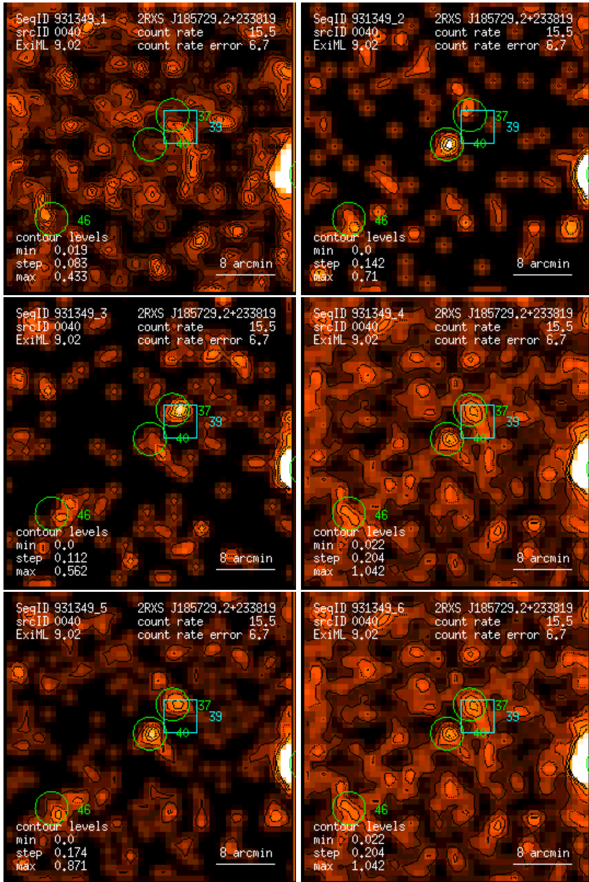
Figure 40: RASS 931349: detection 0040: band rate images, Gaussian filter: (1) PSPC channels 11 – 41, (2) 52 – 90, (3) 91 – 201, (4) 11 – 235, (5) 52 – 201, (6) 11 – 201. Broad band rates in counts/ks. Band rate contour levels in counts/ks/arcmin 2 .
