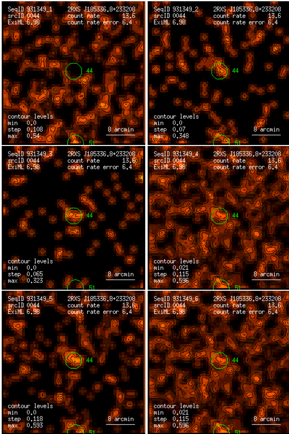
Figure 44: RASS 931349: detection 0044: band rate images, Gaussian filter: (1) PSPC channels 11 – 41, (2) 52 – 90, (3) 91 – 201, (4) 11 – 235, (5) 52 – 201, (6) 11 – 201. Broad band rates in counts/ks. Band rate contour levels in counts/ks/arcmin 2 .
