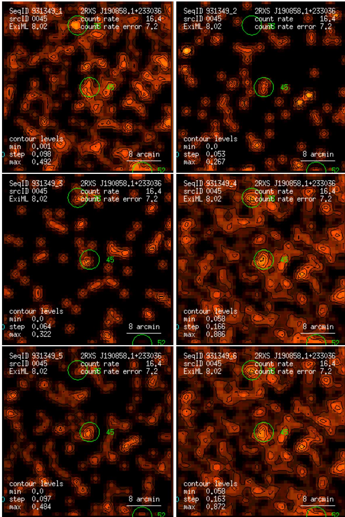
Figure 45: RASS 931349: detection 0045: band rate images, Gaussian filter: (1) PSPC channels 11 – 41, (2) 52 – 90, (3) 91 – 201, (4) 11 – 235, (5) 52 – 201, (6) 11 – 201. Broad band rates in counts/ks. Band rate contour levels in counts/ks/arcmin 2 .
