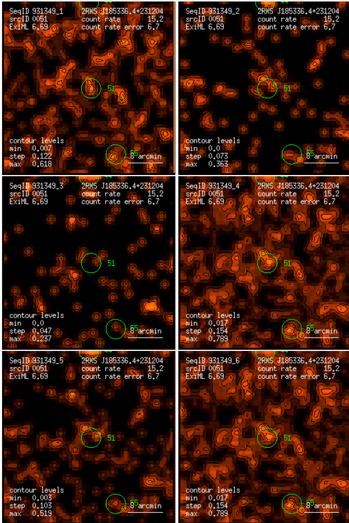
Figure 51: RASS 931349: detection 0051: band rate images, Gaussian filter: (1) PSPC channels 11 – 41, (2) 52 – 90, (3) 91 – 201, (4) 11 – 235, (5) 52 – 201, (6) 11 – 201. Broad band rates in counts/ks. Band rate contour levels in counts/ks/arcmin 2 .
