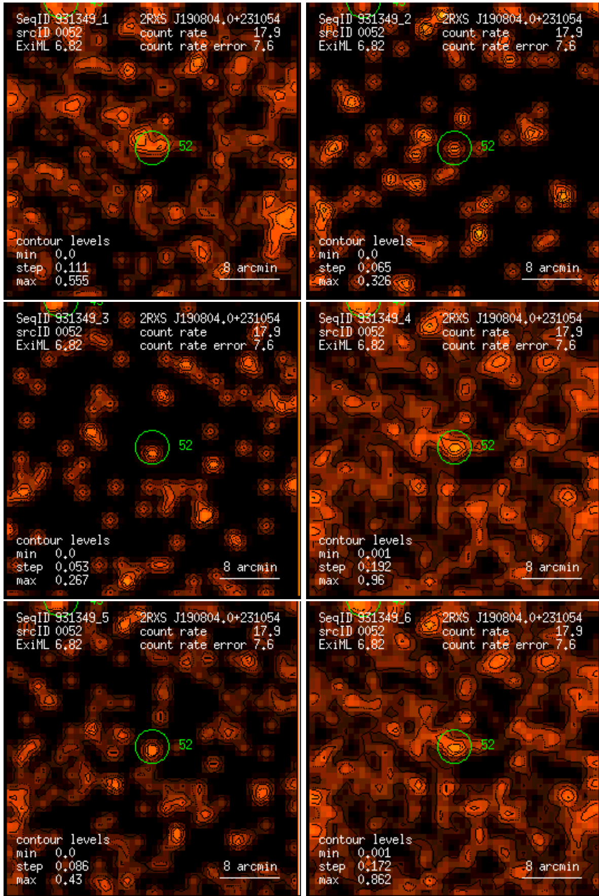
Figure 52: RASS 931349: detection 0052: band rate images, Gaussian filter: (1) PSPC channels 11 – 41, (2) 52 – 90, (3) 91 – 201, (4) 11 – 235, (5) 52 – 201, (6) 11 – 201. Broad band rates in counts/ks. Band rate contour levels in counts/ks/arcmin 2 .
