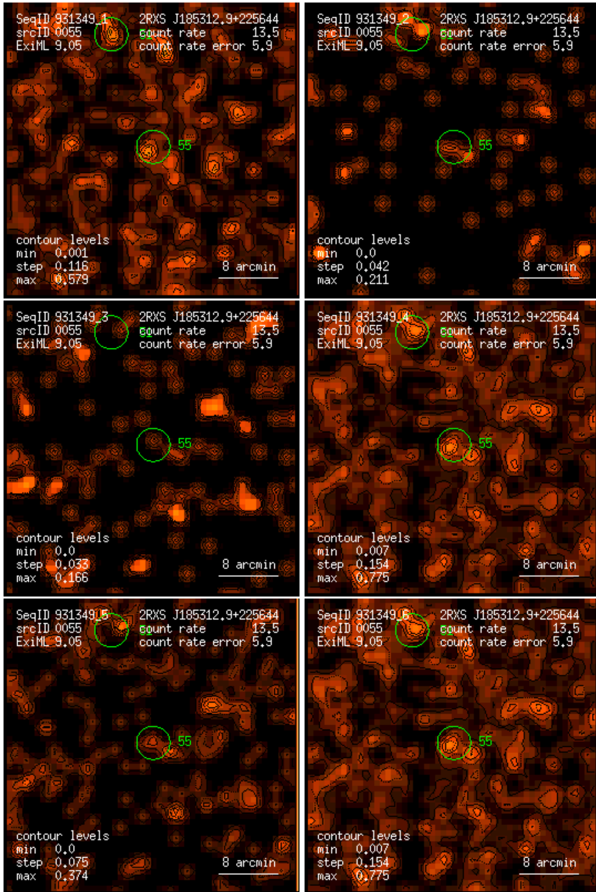
Figure 55: RASS 931349: detection 0055: band rate images, Gaussian filter: (1) PSPC channels 11 – 41, (2) 52 – 90, (3) 91 – 201, (4) 11 – 235, (5) 52 – 201, (6) 11 – 201. Broad band rates in counts/ks. Band rate contour levels in counts/ks/arcmin 2 .
