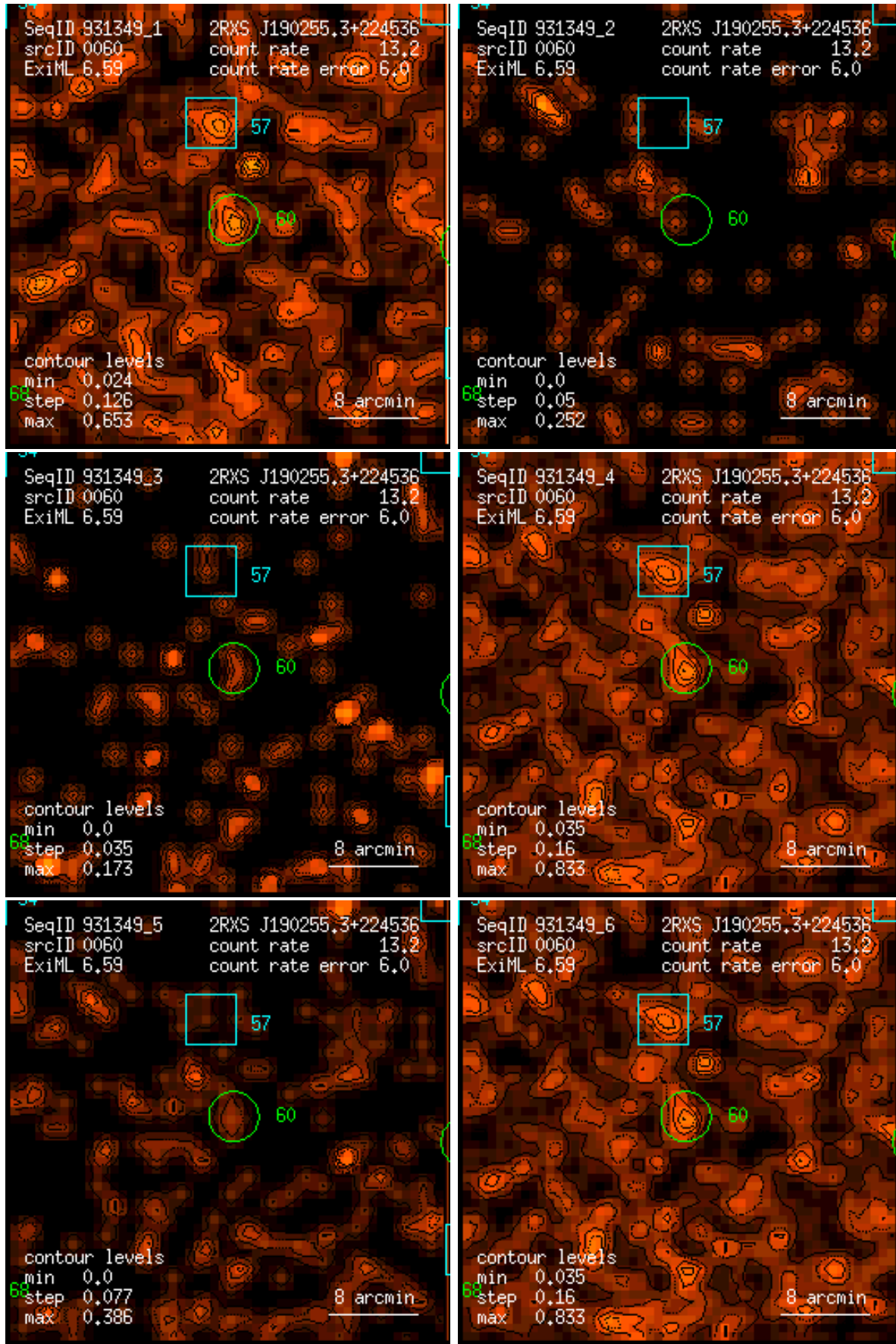
Figure 60: RASS 931349: detection 0060: band rate images, Gaussian filter: (1) PSPC channels 11 – 41, (2) 52 – 90, (3) 91 – 201, (4) 11 – 235, (5) 52 – 201, (6) 11 – 201. Broad band rates in counts/ks. Band rate contour levels in counts/ks/arcmin 2 .
